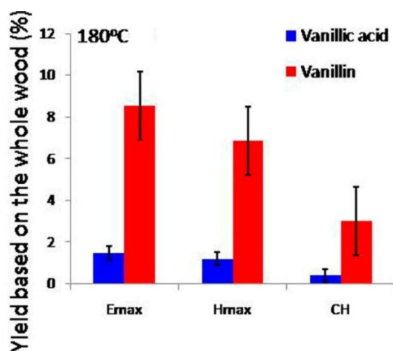
Figure 2. Comparison of the yields to vanillin and vanillic acid by microwave electric ( E_{\max} ) and magnetic ( H_{\max} ) effects and conventional heating (CH) in a cavity perturbation heating system, adapted from [50].
