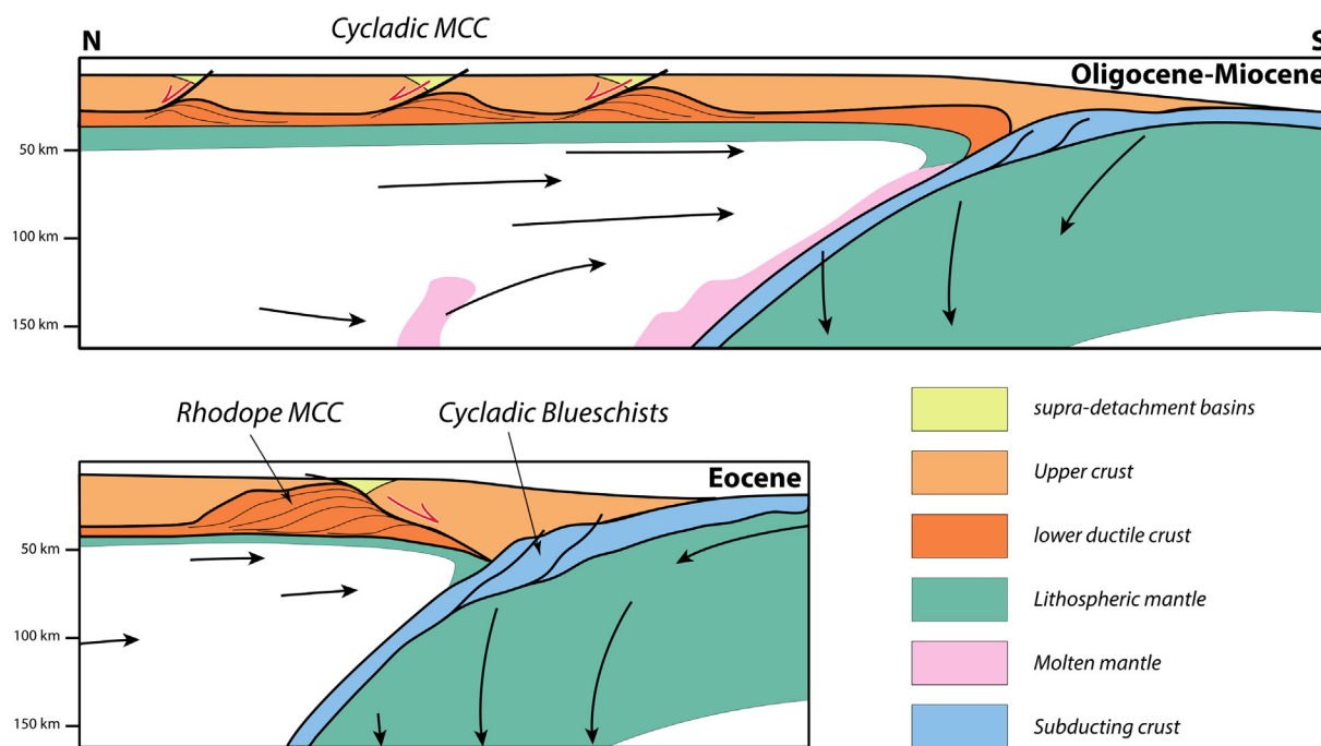
Fig. 4. Schematic cross-sections across the Aegean domain in the Eocene and the Oligo-Miocene showing the main active MCCs and detachments.
