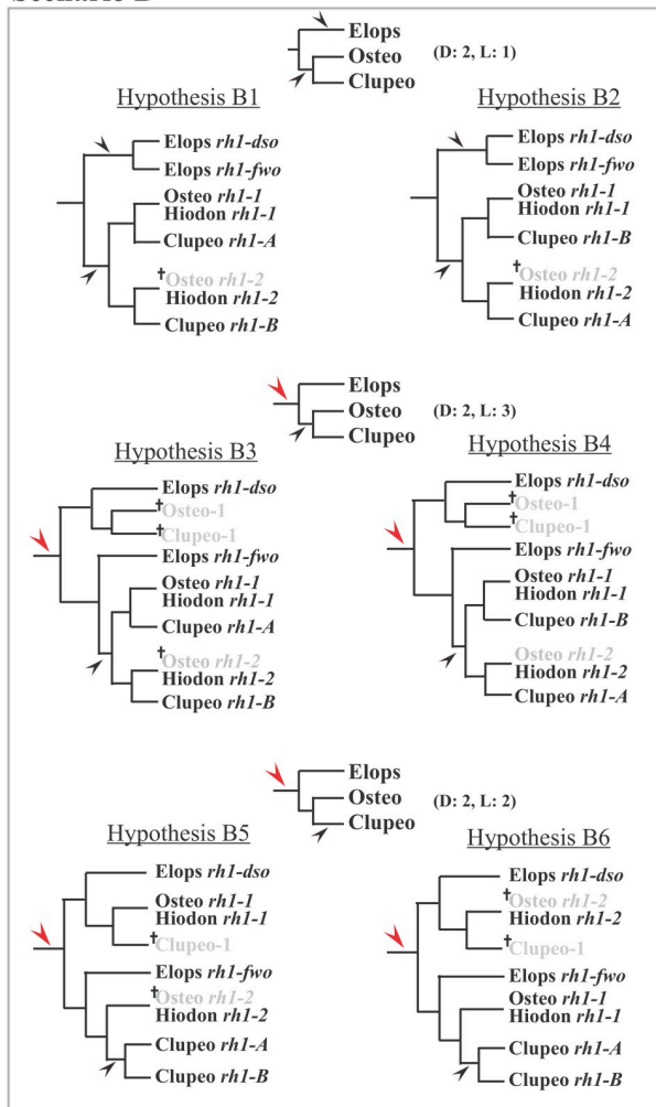
Fig 3. Alternative hypotheses of rh1 gene evolution in the Teleostei. Scenario A, B, and C imply that the major gene duplication events occurred three times, twice, and once, respectively. Observed gene lineages are defined according to the rh1 gene tree (see the annotation
