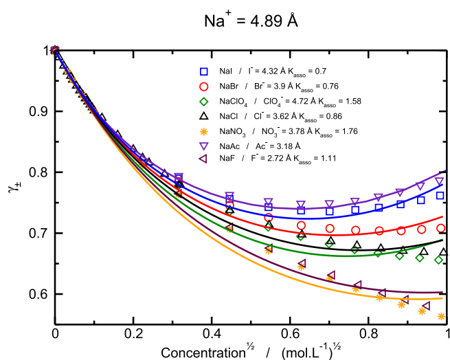
Fig. 1. The mean activity coefficient of sodium salt as a function of square root of the total salt molar concentration.
