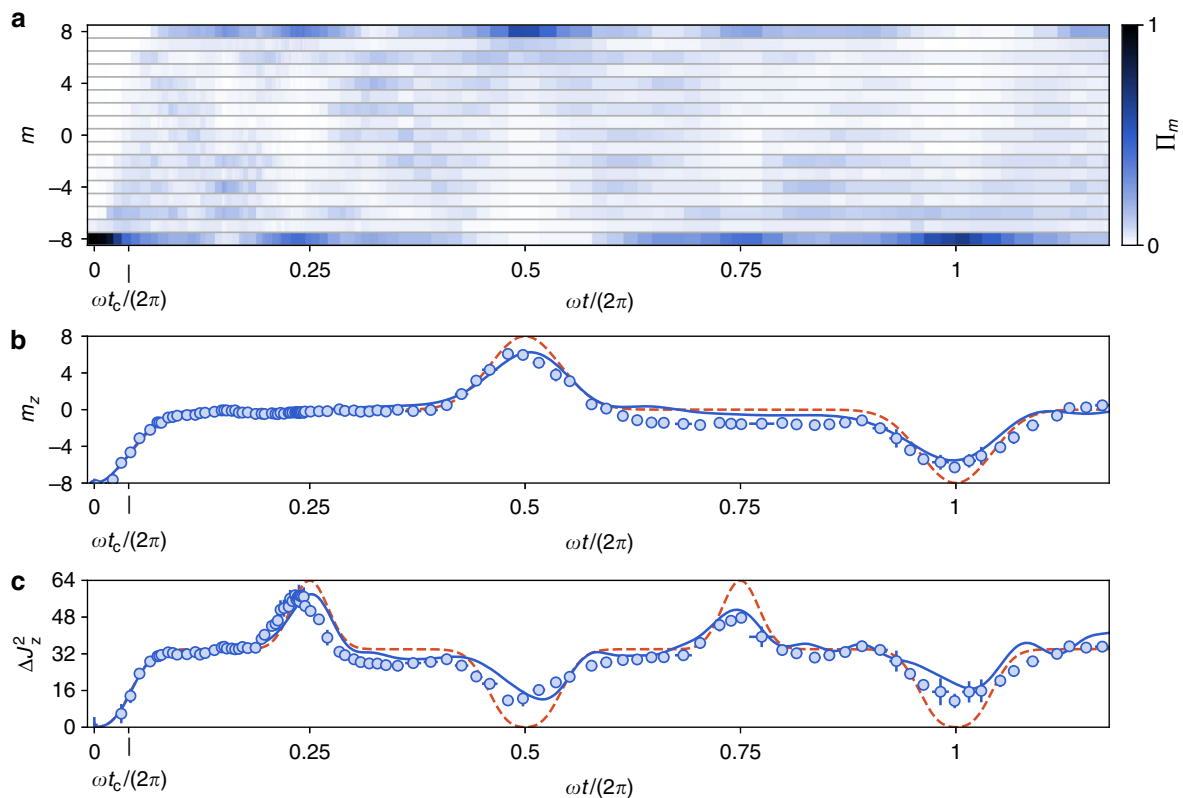
Fig. 2 Collapses and revivals in the non-linear spin dynamics. a Evolution of the spin projection probabilities \Pi_m along z as a function of the light pulse area \omega t_c . b, c Evolution of the magnetization m_z and of the variance in the spin projection \Delta J_z^2 calculated from the \Pi_m distributions. The dashed red lines represent the ideal evolution for a \hat{J}_x^2 coupling 43 , and the blue solid lines correspond to a fit taking into account experimental imperfections (see Methods). Each point is the average of five measurements, and the error bars represent the 1\sigma statistical uncertainty
