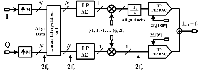
Fig. 6. Proposed transmitter architecture based on 2-path parallel 1-bit HP FIR DACs.
