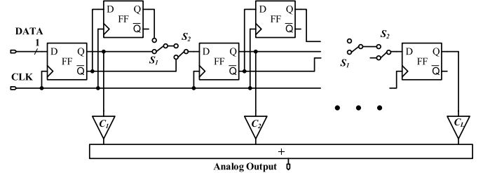
Fig. 11. Configurable delay line for FIR DAC center frequency translation.
