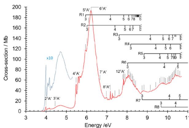
Figure 2. Quinoline absorption spectrum 3.6–10.7 eV. Bands of the Rydberg series R1–R8 are indicated. The O 0 0 origin bands of the successive π-π* valence transitions m 1 A' ← 1 1 A' (Table 5) are indicated as 2 1 A'...12 1 A'. Vibrational components listed in Table 5 are not indicated, for clarity in the figure.
