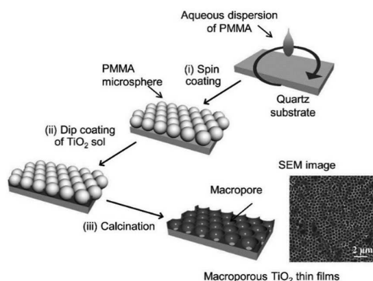
Fig. 16 A schematic diagram of the procedures for the preparation of macroporous TiO 2 thin films. Reproduced from ref. 143 with permission from The Royal Society of Chemistry.
