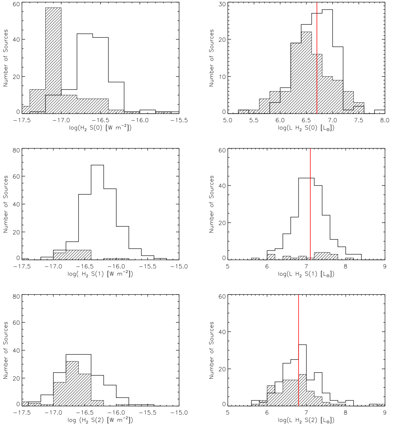
Figure 2. Histograms of measured fluxes (left) and luminosities (right) for the \text{H}_2 molecular gas corresponding to the following rotational transitions, S(0) S(1), and S(2). The fluxes are given in \log[\text{W m}^{-2}] and the luminosities in \log of solar units. Solid histogram present our detections. Dashed histograms show the upper limits, and the red vertical lines indicate the median luminosities.
