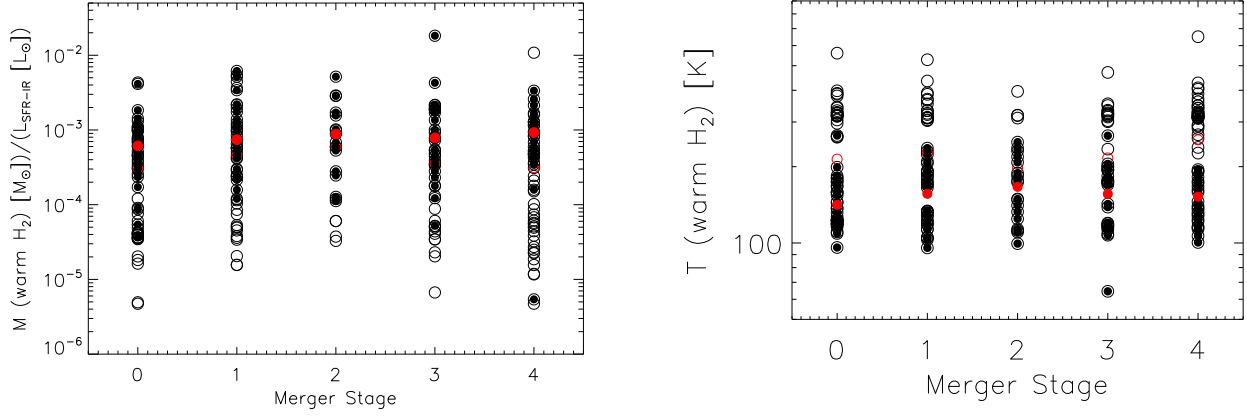
Figure 6. H 2 masses normalized by the L_{\text{IR}} (left) and temperatures (right) versus merger stage. Filled circles use S(0) detections, empty circles use S(0) upper limits. Red circles give the average value for each merger stage.
