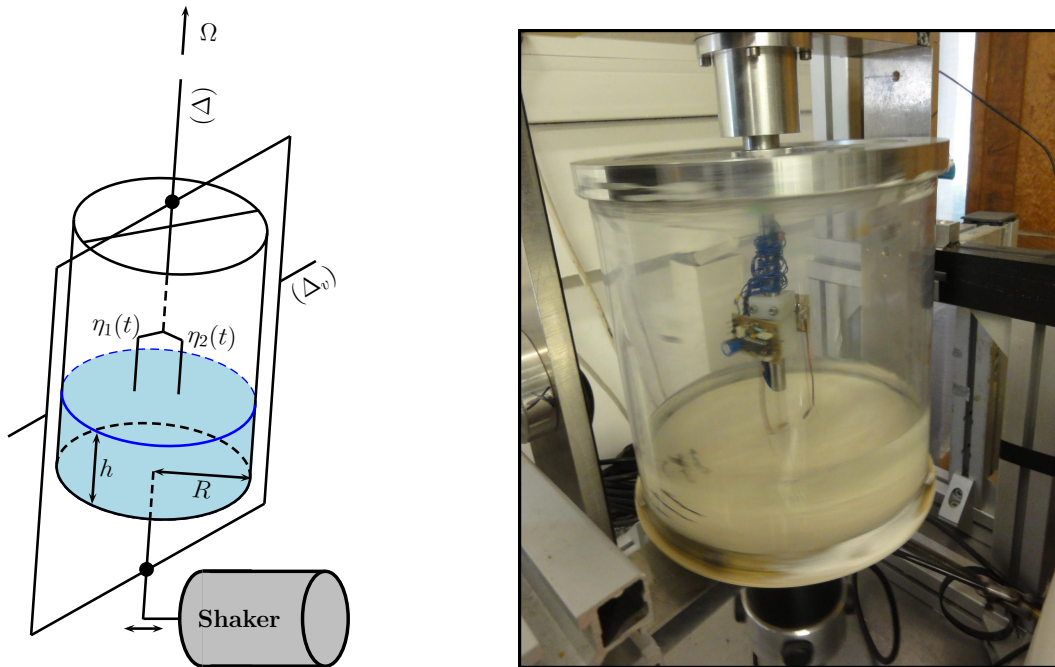
FIG. 1. Experimental setup (sketch and photography). The notations (r, \theta, z) in the text correspond to the usual cylindrical coordinate with z = 0 at the interface. In this experiment, h \simeq 3 cm and R \simeq 9 cm, while a typical value of \Omega is 2\pi \times 250 mHz.
