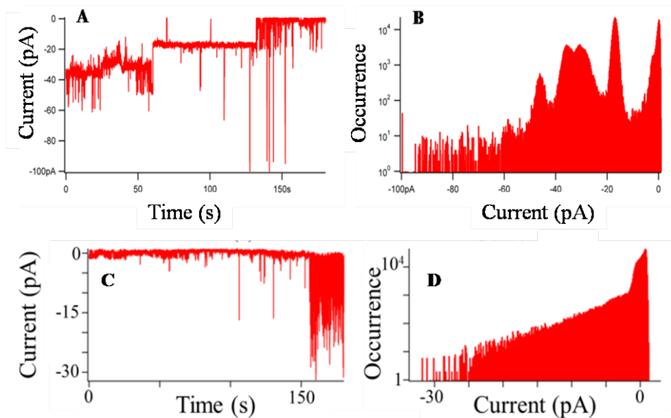
Figure S8. Electrical traces obtained in presence of CD-PEG3 (0.2 \mu M-KCl 1M)
