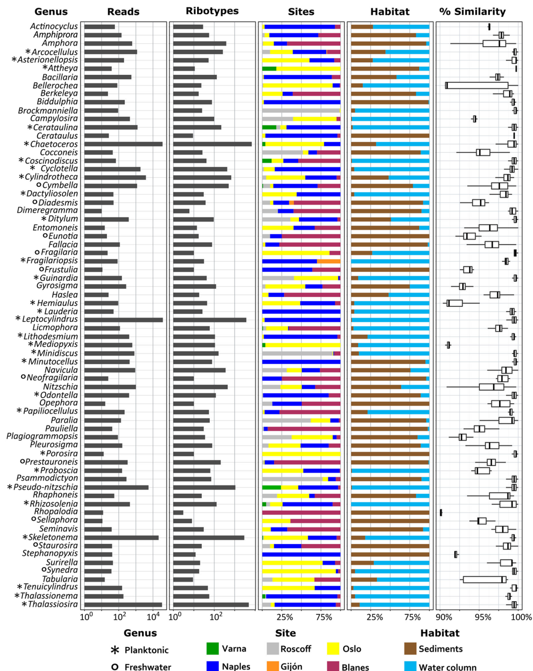
Figure 2. Abundance and distribution of the main diatom genera at coastal European sites. All ribotypes (summing all habitats, size fractions and templates) are clustered at genus level and only the 70 genera represented by more than 9 reads are shown. The colour scheme for the sites reflects the one of Fig. 1b. The rightmost column shows the similarity of the reads to known reference sequences of the genera.
