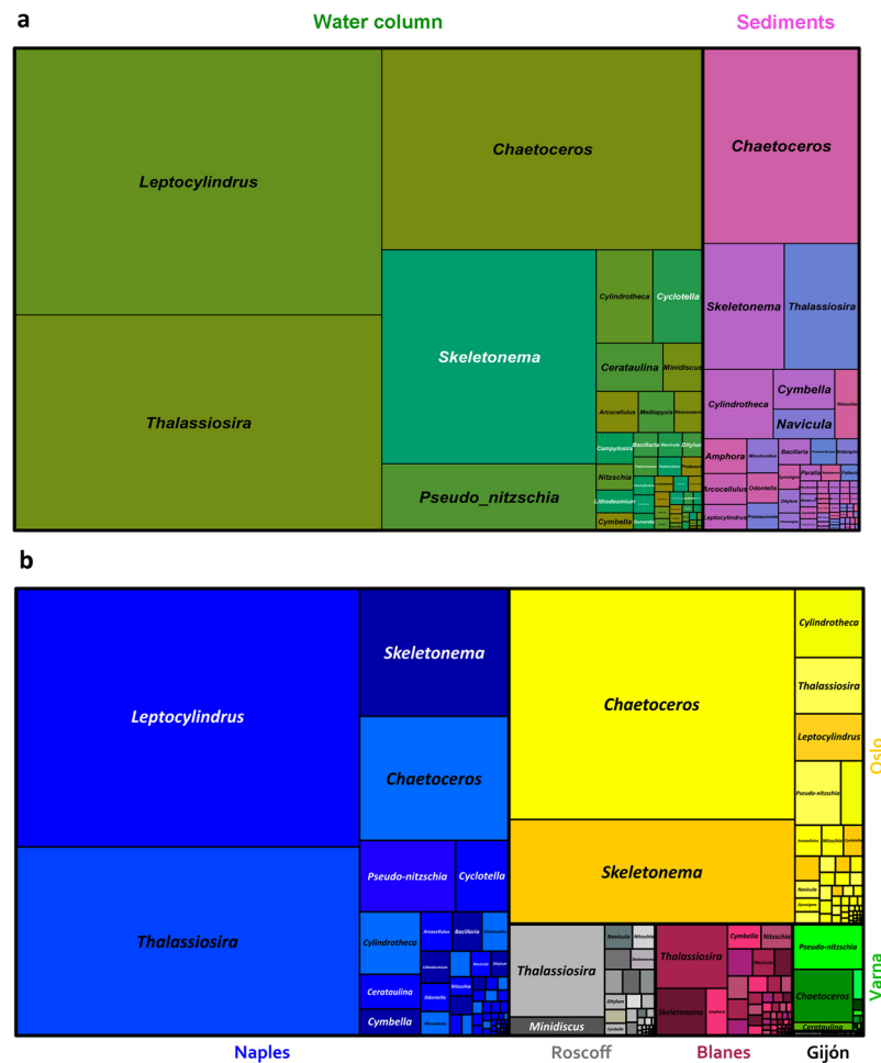
Figure 1. Distribution of diatom genera in coastal European seas. (a) Distribution of genera in the whole water column (green nuances) and sediment (pink nuances) datasets, both dominated by planktonic genera ( Leptocylindrus , Chaetoceros , Thalassiosira and Skeletonema ). (b) Different contribution of diatoms and relative abundance of main genera (including water column and sediments) at European sampling sites (Naples = blue, Oslo = yellow, Roscoff = grey, Blanes = purple, Varna = green, Gijón = black). Naples and Oslo samples collected in two different seasons were merged.
