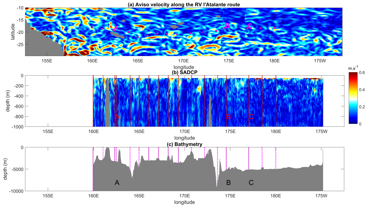
Figure 2. Surface geostrophic currents inferred from AVISO altimetric data, (a); longitude-depth section of 38kHz SADCPC velocity modulus, (b); bathymetry along the RV I'Atalante route, (c); VMP stations are displayed with magenta circles in (a) and with vertical dashed red lines in (b) and magenta lines in (c).
