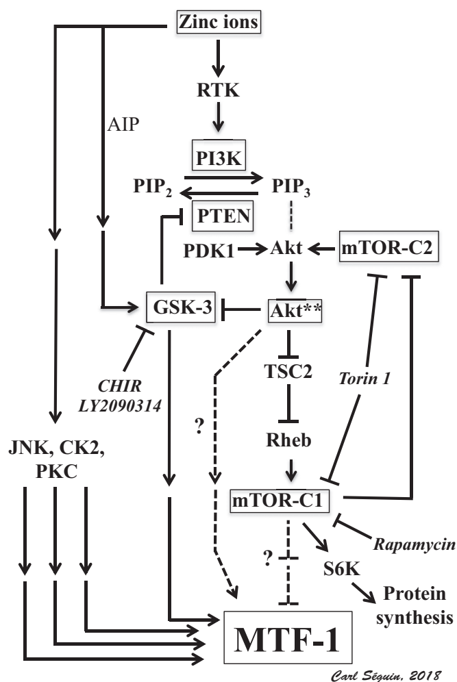
Fig. 5. Putative model of the signaling pathways involved in the activation of MTF-1. Zinc ions activate a receptor tyrosine kinase (RTK), which recruits and activates PI3K. PI3K then produces PI(3,4,5)P 3 , which serves as a docking site for Akt and PDK1. Akt is phosphorylated by mTOR in complex 2 and PDK1. The activated Akt (Akt ** ) dissociates from the membrane and phosphorylates various target proteins including GSK-3 and TSC2, a negative regulator of Rheb, a RAS-related GTPase. Active Rheb helps activate mTOR in complex 1, thereby promoting protein synthesis by phosphorylating p70S6 kinase (S6K). Full activation of MTF-1 in response to zinc ions also requires the action of the JNK, CK2, and PKC signaling transduction pathways (LaRoche et al. 2001; Saydam et al. 2002). Activation of MTF-1 by the PI3K pathway may involve an Akt signal transduction pathway targeting MTF-1 (broken arrows), or the inhibition by mTOR-C1 of a putative inhibitory protein (broken lines, downstream of mTOR-C1). We show here that GSK-3 is involved in the activation of MTF-1 through an Akt-independent positive regulatory pathway (AIP). Activated GSK-3 could directly phosphorylate and activate MTF-1, or could affect MTF-1 through a signaling pathway converging on MTF-1. Alternatively, GSK-3 could affect MTF-1 by its inhibitory action on PTEN which antagonizes the PI3K signaling pathway. In addition, PTEN (Lin et al. 2012) and PP2A (Chen et al. 2014) (not illustrated) have been shown to interact with MTF-1 and regulate its activity. The kinases targeted by CHIR99021 (CHIR), LY2090314, Torin 1 and rapamycin are indicated. The question marks indicate putative pathways.
