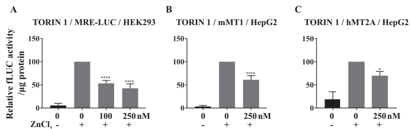
Fig. 1. Effect of Torin 1 on (MREd) 6 -LUC (MRE-LUC) (A), MT1-LUC (mMT1) (B), and MT2A-LUC (hMT2A) (C) expression. HEK293 (A) and HepG2 (B and C) cells transfected with the different reporter plasmids, as indicated, were serum-starved and pre-incubated for 30 min with the vehicle alone (0) or with 100 or 250 nmol/L of Torin 1, as indicated below the graphs, and then treated or not with 100 μmol/L ZnCl 2 for 16 h. Cell extracts were prepared, and measurement of LUC activity was performed with a dual LUC kit. Results are expressed as firefly LUC (fLUC) activity per microgram (μg) of total protein, and as a percentage relative to that of the control induced by zinc, which is taken as 100%. The data represent the mean ± S.D. of 3 independent experiments performed in triplicate. Significant differences between the control and treated samples are based on the one-way ANOVA followed by a Bonferroni post-hoc test (*, p \leq 0.05 ; ****, p < 0.0001 ).
