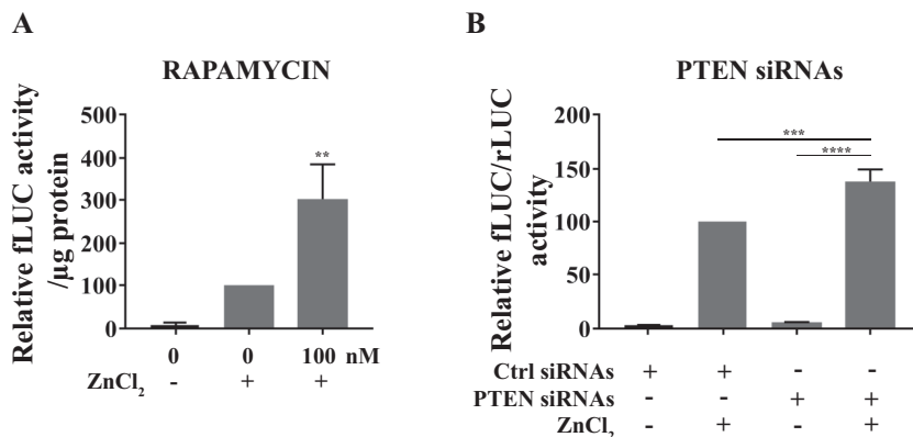
Fig. 2. Effect of rapamycin (A) and PTEN siRNAs (B) on (MREd) 6 -LUC expression. (A) HEK293 cells transfected by the PEI method with the reporter plasmids were serum-starved and preincubated for 30 min with the vehicle alone (0) or with 100 nmol/L of rapamycin, as indicated, and then treated or not with 100 μmol/L ZnCl 2 for 16 h. Cell extracts were prepared, and measurement of LUC activity was performed as indicated in Fig. 1. (B) HEK293 cells transfected by the calcium phosphate method with a mixture of (MREd) 6 -LUC and pTK-rLUC as internal standard together with 250 ng of negative control (Ctrl) or PTEN siRNAs were serum-starved and then treated, or not, with 100 μmol/L ZnCl 2 for 16 h. Cell extracts were prepared, and measurement of LUC activity was performed with a dual LUC kit. Results are expressed as percentage firefly LUC (fLUC) activity relative to the level directed by the Renilla LUC (rLUC) construct. The data represent the mean ± S.D. of 3 independent experiments performed in triplicate. Significant differences between the control and treated samples are based on the one-way ANOVA followed by a Bonferroni post-hoc test (**, p \leq 0.01 ; ***, p \leq 0.001 ; ****, p < 0.0001 ).
