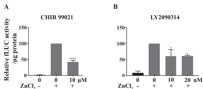
Fig. 4. Effect of CHIR99021 (A) and LY2090314 (B) on (MREd) 6 -LUC expression. HEK293 cells transfected with the reporter plasmid were serum-starved and pre-incubated for 30 min with the vehicle alone (0) or with 10 \mu mol/L of CHIR99021, or 10 or 20 nmol/L of LY2090314, as indicated, and then treated or not with 100 \mu mol/L ZnCl 2 for 16 h. Cell extracts were prepared, and measurement of LUC activity was performed as indicated in Fig. 1. Results are expressed as relative firefly LUC (fLUC) activity per microgram ( \mu g) of total protein, and as a percentage relative to that of the control induced by zinc, which is taken as 100%. The data represent the mean \pm S.D. of 3 independent experiments performed in triplicate. Significant differences between the control and treated samples are based on the one-way ANOVA followed by a Bonferroni post-hoc test (*, p \leq 0.05 ; ****, p < 0.0001 ).
