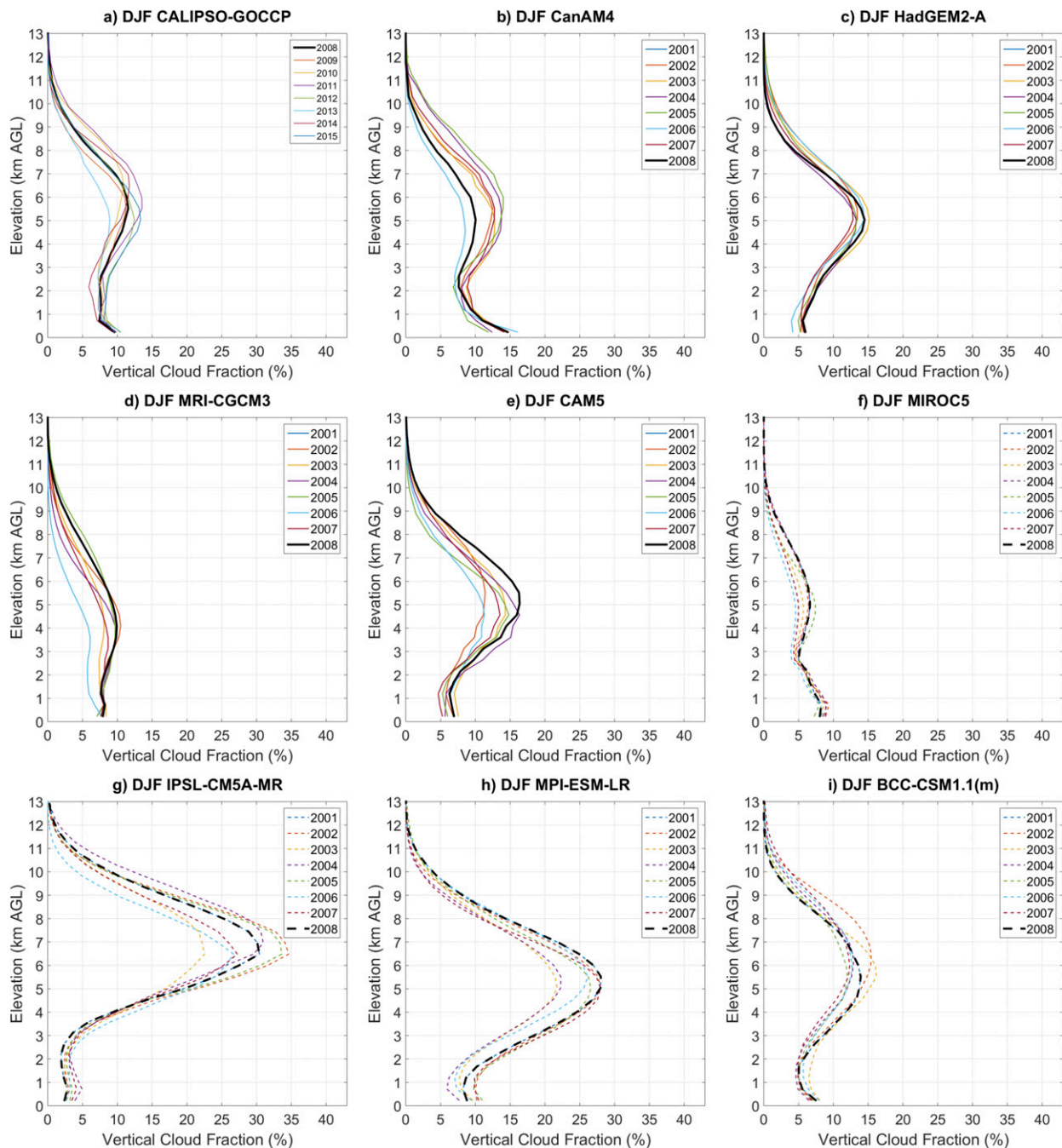
FIG. 7. Mean cloud fraction profile over Greenland calculated in DJF for (a) CALIPSO-GOCCP for the years 2008–15 and for (b)–(i) eight CMIP5 models for the years 2001–08.
