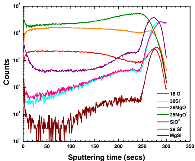
FIGURE 4 Secondary ion mass spectroscopy (SIMS) spectra of magnesium oxide (MgO) thin film
