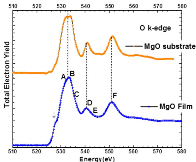
FIGURE 1 X-ray absorption spectra of 500-Å-thick MgO thin film and that of a MgO substrate measured in total electron yield mode near the O-K absorption edge region
