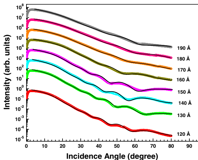
FIGURE 2 Measured (star) and fitted (continuous solid line) angle-dependent soft X-ray reflectivity curve of magnesium oxide (MgO) thin film over the wavelength range of 120-190 Å
