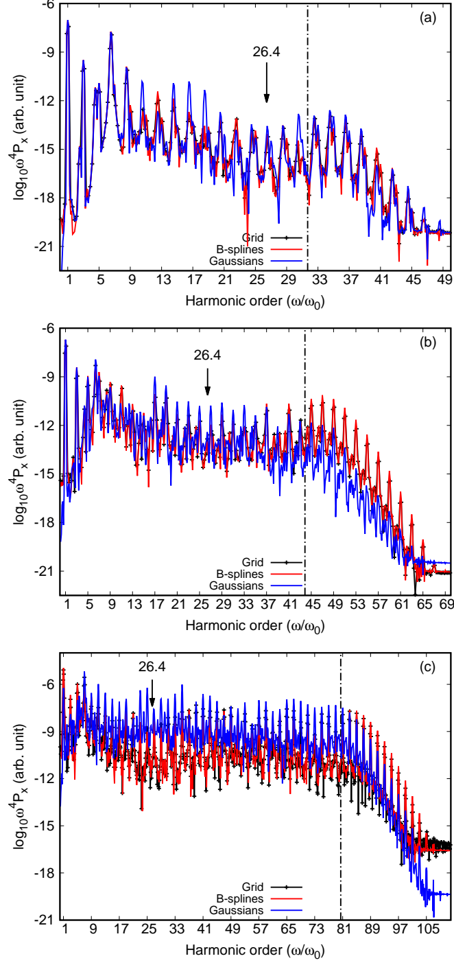
Figure 4: HHG spectra calculated from the electron dipole at the equilibrium internuclear distance R = 2.0 au with laser intensities: (a) I = 10^{14} W/cm 2 , (b) I = 2 \times 10^{14} W/cm 2 , and (c) I = 5 \times 10^{14} W/cm 2 . Intensities I = 5 \times 10^{13} and 7 \times 10^{14} W/cm 2 are reported in the Supplementary Information. For each HHG spectrum, the dot-dashed lines indicate the cutoff energies, which are given by the rescattering model as E_{\text{cutoff}} = I_p + 3.17U_p , see Ref.: 60,61 (a) E_{\text{cutoff}} = 31.7\omega_0 , (b) E_{\text{cutoff}} = 43.9\omega_0 , and (c) E_{\text{cutoff}} = 80.5\omega_0 . The arrow points to the expected position of the two-center interference minimum extracted from the recombination dipole.
