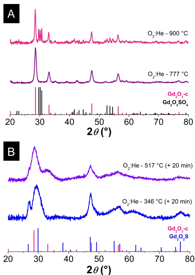
Figure 7: Powder XRD patterns of annealed \text{Gd}_2\text{O}_2\text{S} nanoplates under \text{O}_2:\text{He} (20/80 v/v), (A) at 900 °C (pink) and 777 °C (purple), (B) 517 °C (violet) and 346 °C (blue). In (A) the heating was stopped once the target temperature was reached. In (B), the target temperature was maintained for 20 min before cooling down. XRD pattern references are JCPDS files 26-1422 ( \text{Gd}_2\text{O}_2\text{S} , blue), 12-0797 ( \text{Gd}_2\text{O}_3 -cubic, pink) and 77-9842 ( \text{Gd}_2\text{O}_2\text{SO}_4 , black).
