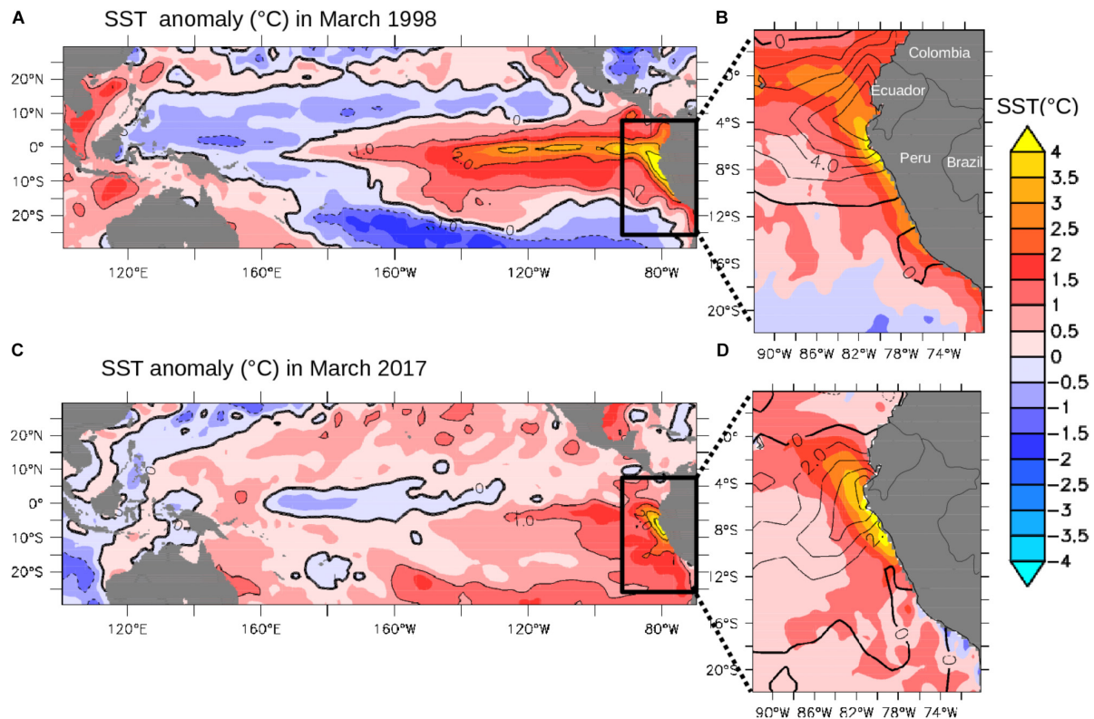
FIGURE 1 | (A) SST anomaly (in °C) and (B) SST anomaly (in °C, color scale) and precipitation (in mm day -1 , contours) during the 1997–1998 El Niño in March 1998; (C,D) are same as (A,B) during the 2017 coastal El Niño in March 2017. Anomalies were computed with respect to the 1981–2016 climatology.
