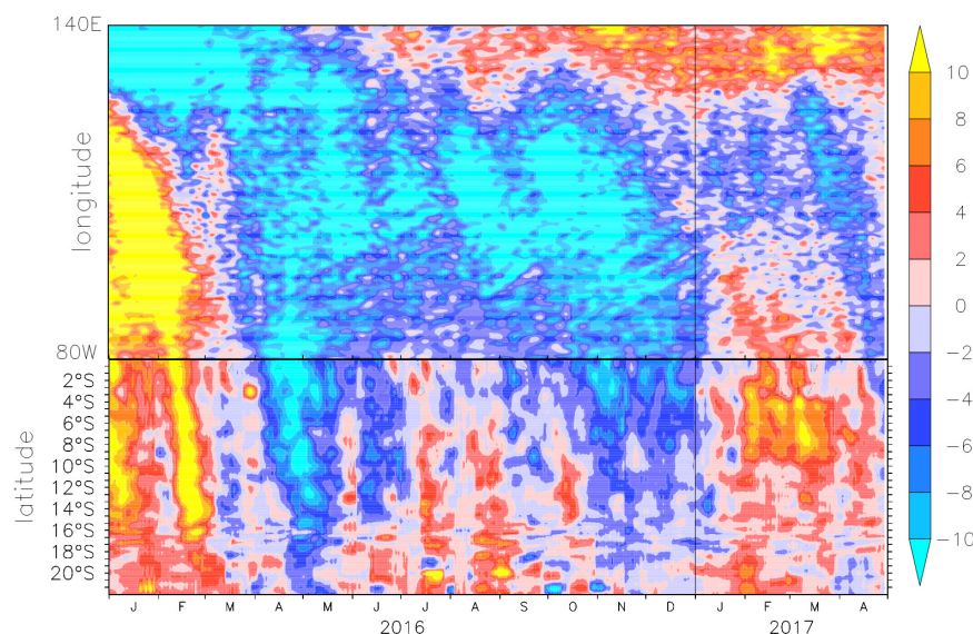
FIGURE 3 | Hovmöller of altimetric sea level anomaly (in cm) along the equator (140°E–80°W) and along the coast of Peru (0°–22°S). The sea level anomalies were computed using the 1/4^{\circ} \times 1/4^{\circ} gridded product, such that for each latitude, the sea level observations were averaged between the coast and 50 km offshore. The anomalies were computed with respect to a 2013–2016 climatology.
