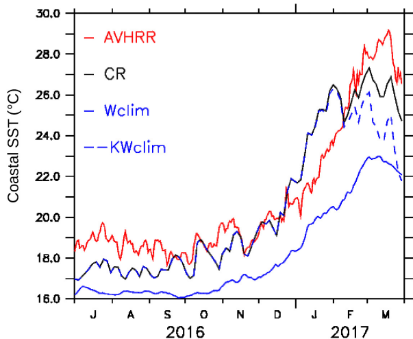
FIGURE 10 | Time evolution of the SST averaged in a coastal box ( 4\text{--}10^{\circ}\text{S} , 0\text{--}100 km from the coast) for AVHRR observations (red line), CR (black line), Wclim (blue line), and KWclim (dashed blue line).
