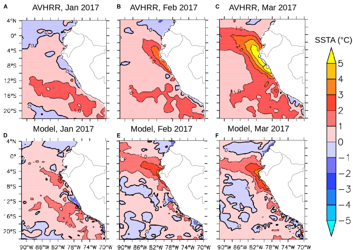
FIGURE 4 | SST anomalies in (A,D) January, (B,E) February, and (C,F) March 2017 from SST observations (top) and model output (bottom). Anomalies were computed with respect to 2013–2016 climatology. The blue line in (C) indicates the location of the Chicama section.
