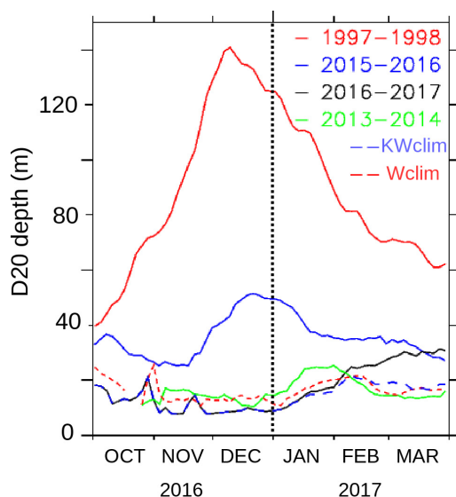
FIGURE 7 | Time evolution of the depth of the 20°C isotherm (D20, in meters) between October (year–1) and March (year+1) for different time periods (see labels). D20 was averaged in a coastal box between 4°S and 10°S and within 200 km from the coast.
