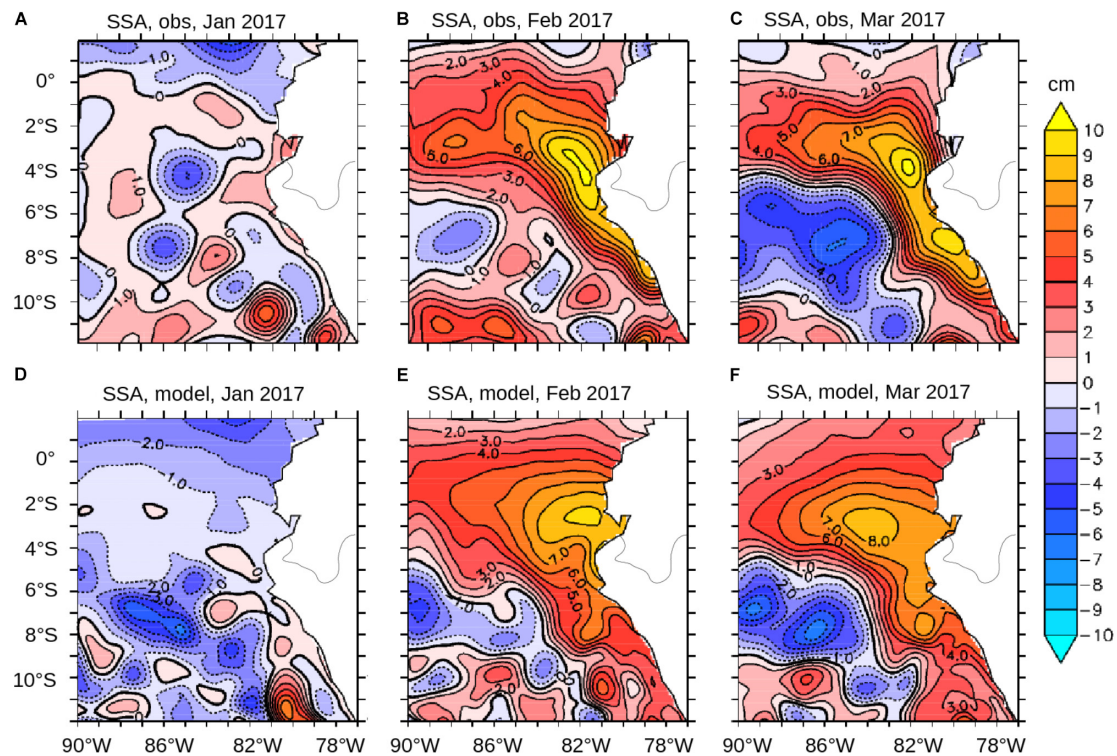
FIGURE 6 | Sea level anomaly (in cm) in (A,D) January; (B,E) February; (C,F) March 2017, from satellite observations (top) and model (bottom). Anomalies were computed with respect to the 2013–2016 climatology.
