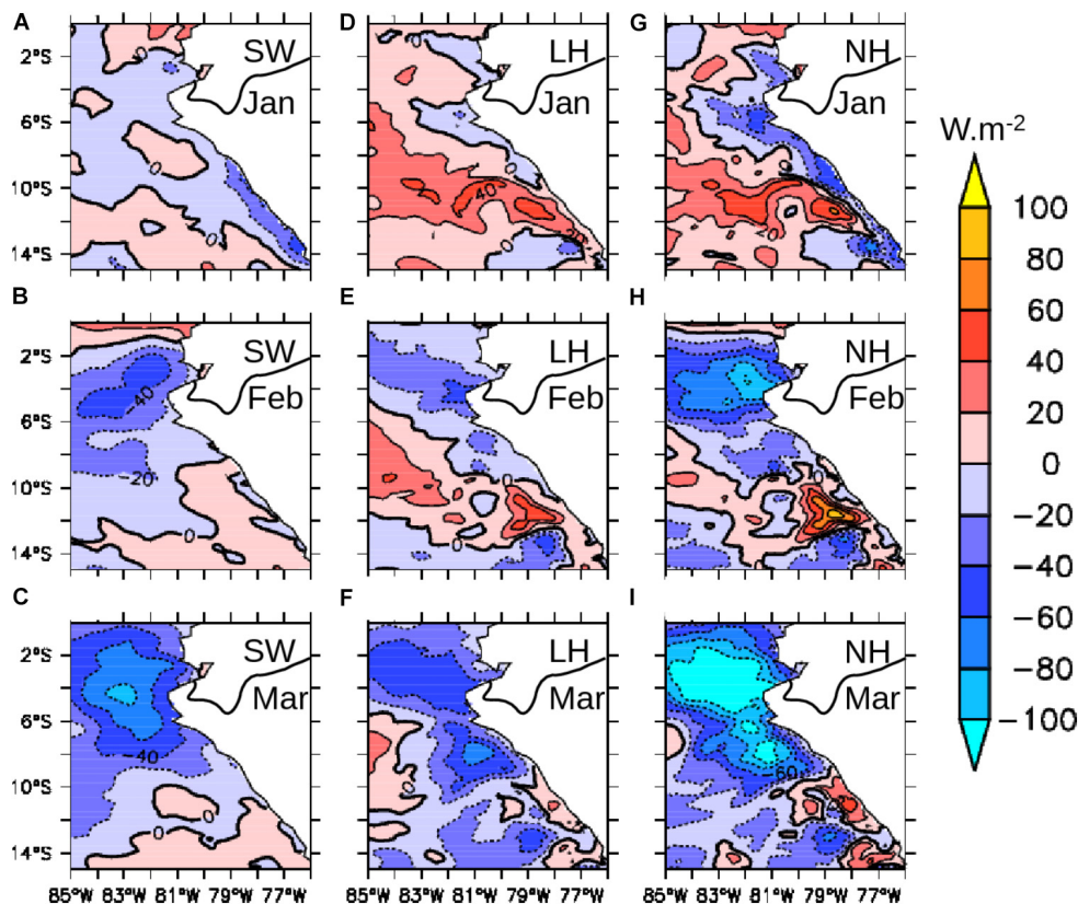
FIGURE 8 | Monthly heat flux anomalies (in \text{W m}^{-2} , positive downward) in January, February, and March 2017: (A–C) short wave heat flux anomaly (SW); (D–F) latent heat flux anomaly (LH); and (G–I) net heat flux anomaly (NH). Positive fluxes indicate an input of heat into the ocean. Anomalies were computed with respect to the 2013–2016 model climatology.
