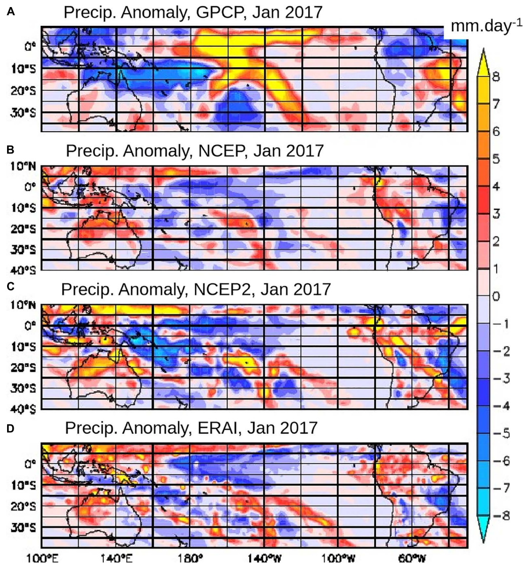
FIGURE 13 | Mean precipitation anomaly (in mm day -1 ) in January 2017 from: (A) GPCP, (B) NCEP, (C) NCEP2, and (D) ERAI. Monthly anomalies were computed over the period 1979–2016.
