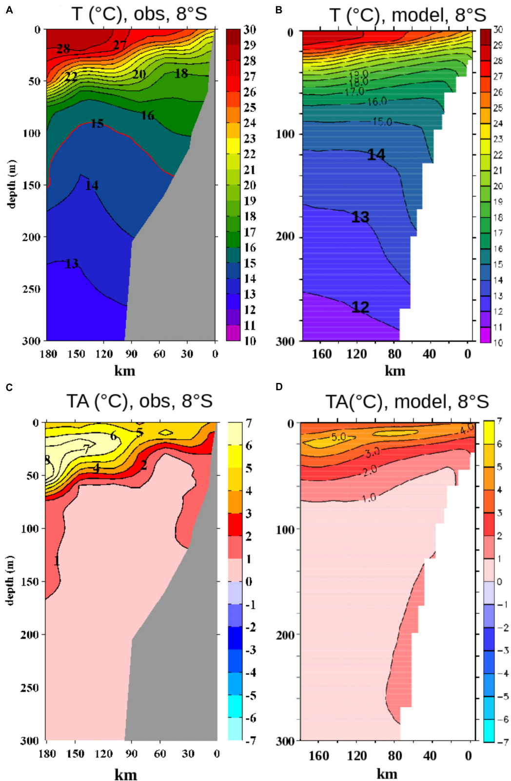
FIGURE 5 | Cross-shore vertical sections of temperature (A,B) absolute values and (C,D) anomalies (in °C) in March 2017 off the northern Peru shelf (Chicama, 8°S). The section's location is indicated in Figure 4C. Observed anomalies (c) were computed with respect to a climatology of IMARPE data for the period 1981–2010, while modeled anomalies were computed with respect to a model climatology for 2013–2016.
