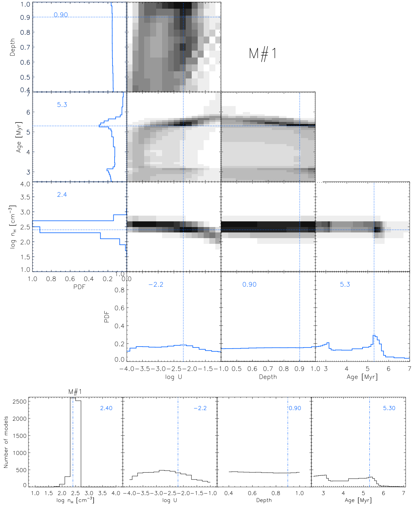
Fig. A.1. Results for the clump M\#1 . Top panels: PDFs for n_{\text{H}} , \log U , t_{\text{burst}} (Age), and physical depth. The blue histograms show the PDF for each single parameter. The 2D PDFs are shown as density plots (black \sim 1 , to white \sim 0 ) at the intersection between two parameters. The blue horizontal and vertical lines indicate the parameter value corresponding to the best model solution, with the corresponding parameter value given in blue. Bottom panels: histograms of parameter distributions for the best models (see text for details).
