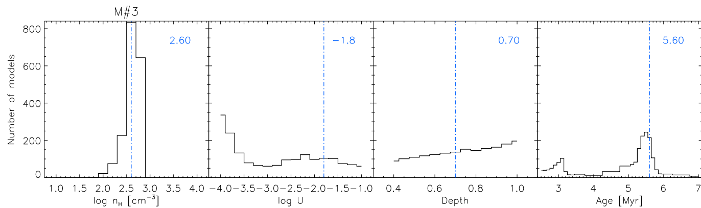
Fig. C.2. Results for the clump M#3 . See Fig. A.1 for the plot description.
