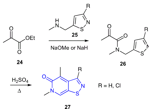
Scheme 8 Synthesis of 5 H ,6 H [1,2]thiazolo[5,4- c ]pyridine-5-ones using an intramolecular dehydrative cyclization
