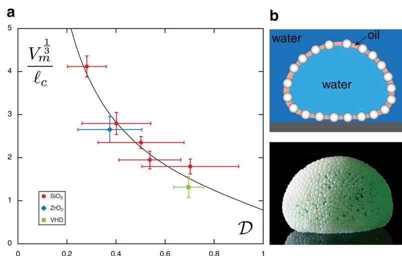
Figure 5. (a) Maximum drop volume as a function of D for various rafts. The black line is the theoretical prediction from the model. (b) Schematic and picture of an armored capsule (water dyed green) after a forced raft destabilization ( \text{SiO}_2 , d = 500 \mu\text{m} ).
