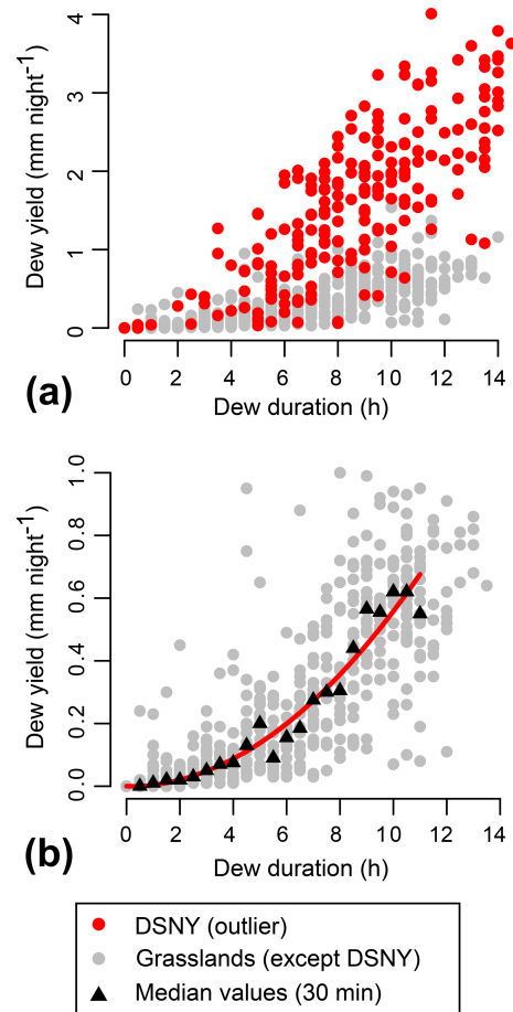
Figure 5. Dew yield versus dew duration for the grasslands (top of the canopy, nightly timescale). (a) shows the failure of the Monin–Obukhov Similarity Theory for DSNY, which is why the quadratic fit ( y = a \times x^2 , a = 0.0056 \text{ mm h}^{-2} , r^2 = 0.94 ) has been calculated for the other grasslands based on the 30 min median values for dew durations between 1 and 11 h (b).
