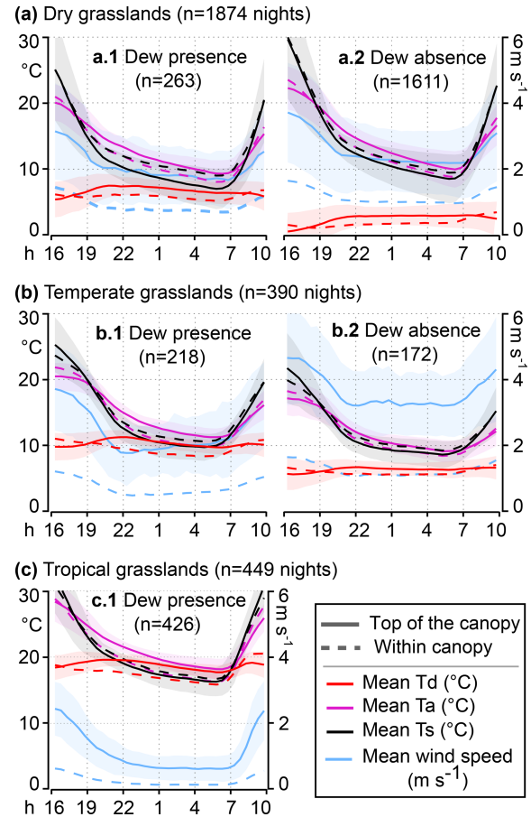
Figure 9. Nocturnal cycles for three populations of grasslands with the mean value of meteorological parameters calculated on a stack of n nights ( n indicated in parenthesis). The solid lines represent the top of the canopy, and the dashed lines represent within canopy. The shaded areas indicate \pm 1 standard deviation of the mean, shown for the top of the canopy only (for visualization purposes). (a.1), (b.1), and (c.1) are based on nights with dew formation, and (a.2) and (b.2) are based on nights without dew formation. (c.2) is missing because of a sample size that is too small.
