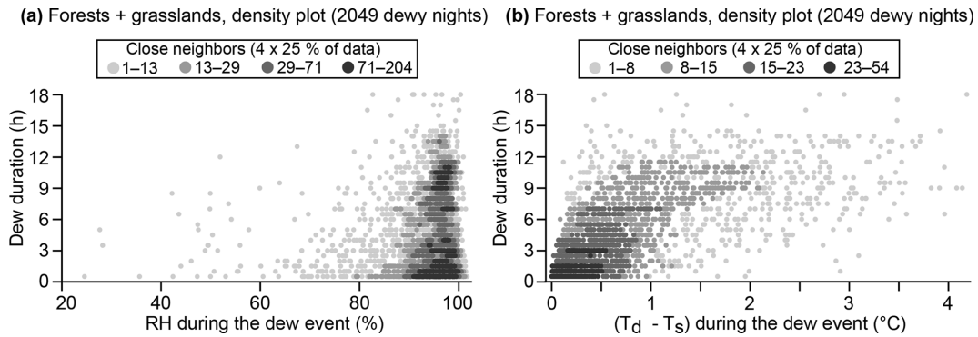
Figure 7. Density plot on a nightly timescale of the dew duration versus relative humidity (a) and dew duration versus T_d - T_s (b), both averaged over the dew duration (all sites included). Four shades of grey indicate the number of neighbors around a data point in a small rectangle ( \sim 2\% of the figure). Each shade of grey represents 25% of the total number of nights.
