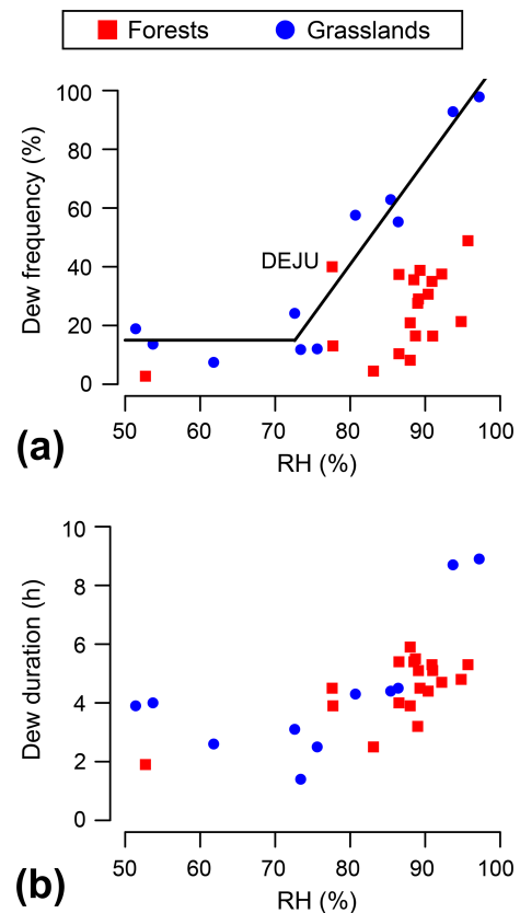
Figure 4. Dew frequency (a) and duration (b) versus RH (from 23:00 to 05:00 the next day) for each site over the growing season. The slope of 3.5 ( r^2 = 0.92 ) in (a) has been calculated based on the grasslands with \text{RH} > 70\% only. Dew formation has been calculated at the top of the canopy of the grasslands and within canopy of the forests only.
