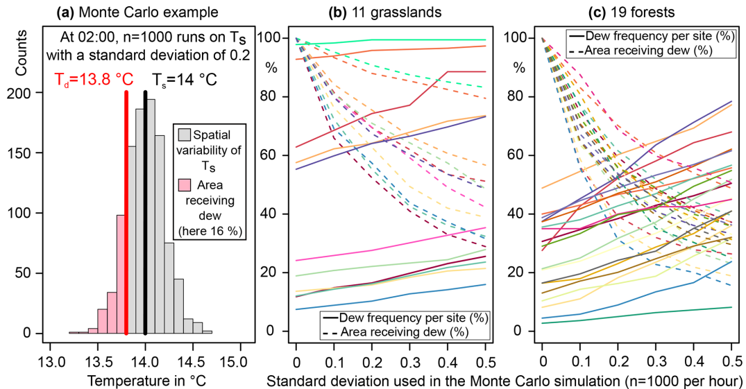
Figure 11. Sensitivity of dew frequency to the spatial variability in the surface temperature based on a Monte Carlo simulation run on each half-hour data point ( n = 1000 runs). The spatial variability is assumed to follow a normal distribution, and only a certain percentage of the canopy will receive dew formation (example for a , 16% at 02:00). The Monte Carlo simulation has been run with different standard deviations (from 0 to 0.5) for each half-hour for all grasslands ( b ) and all forests ( c ). A non-dew event is defined here as less than 5% of the canopy receiving dew formation; then all the areas above 5% have been averaged for each site (dashed lines). Colors allow association between the solid lines and the dashed lines for each site.
