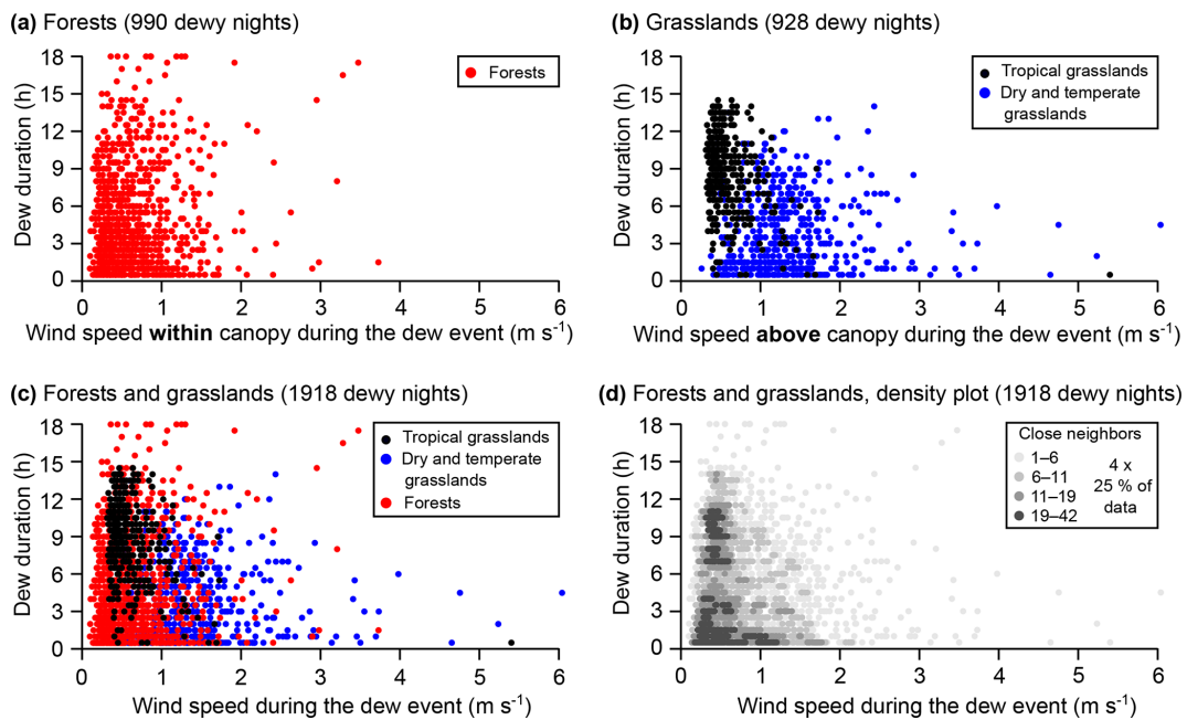
Figure 8. Dew duration versus wind speed averaged during a dew event for different groups (nightly timescale): forests (a; wind speed within canopy), grasslands (b; wind speed 1 m above canopy), both of these (c) and density plot of both (d). In the density plot, four colors indicate the number of neighbors around a data point in a small rectangle ( \sim 2\% of the figure). Each color represents 25% of the total number of nights.
