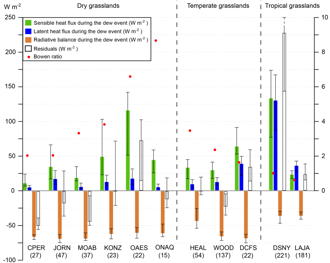
Figure 6. Median value and [25, 75] % quantiles (error bars) of the net radiation above canopy ( R_n ), and the sensible ( H ) and latent heat fluxes ( LE ) averaged during a dew event for each dewy night (indicated in parenthesis). The sign convention is positive when the grassland receives energy, and the residuals are R_n + LE + H , with R_n measured and LE and H calculated with the Monin–Obukhov similarity theory.
