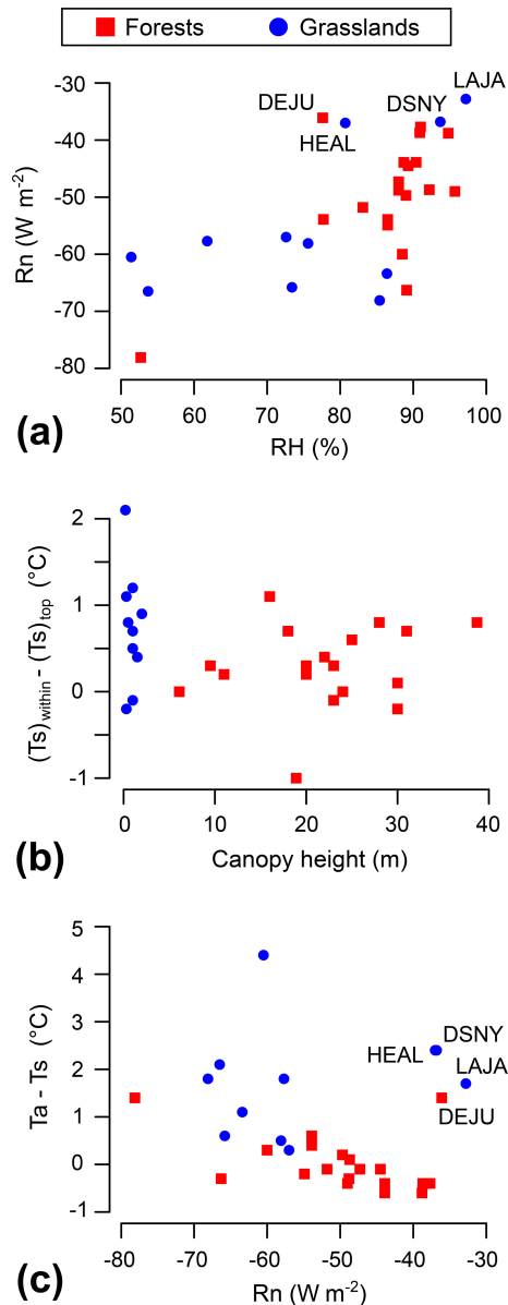
Figure 3. Mean values from 23:00 to 05:00 the next day for each site over the growing season for the following parameters: R_n versus RH (a), difference in T_s between the canopy within and the top of the canopy versus the canopy height (b), and T_a - T_s (within canopy for the forests, top of the canopy for the grasslands) versus R_n (c). Four sites are selected for discussion.
