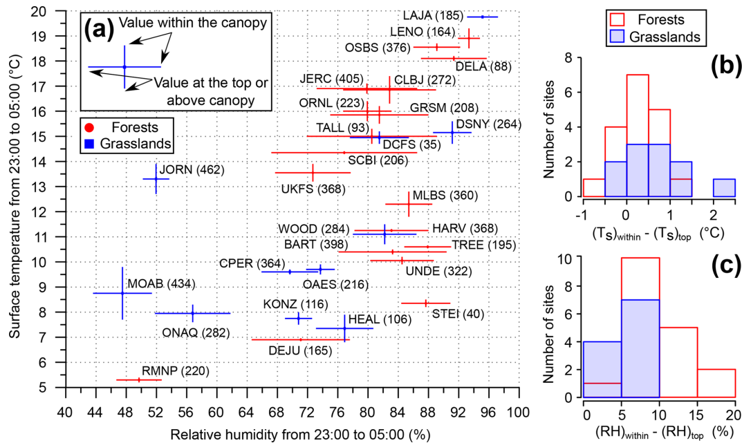
Figure 2. (a) T_s versus RH from 23:00 to 05:00 the next day over the growing season for each site (number of nights is indicated in parenthesis). Four mean values have been calculated per site, two from the sensors within canopy and two from the sensors at the top of canopy. (b, c) Histograms of the difference in T_s (and RH) between that within canopy and that at the top of the canopy. SERC is missing because of a sensor failure above canopy.
