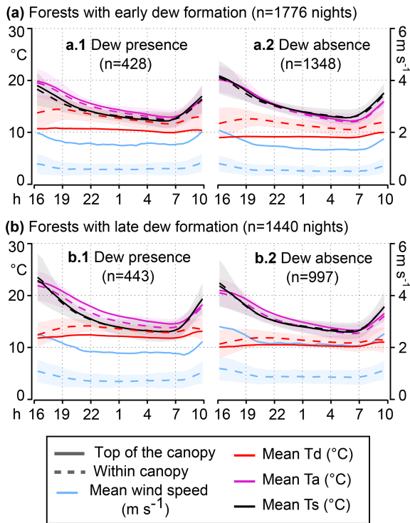
Figure 10. Nocturnal cycles for two populations of forests with the mean value of meteorological parameters calculated on a stack of n nights ( n indicated in parenthesis). The solid lines represent the top of the canopy, and the dashed lines represent within canopy. The shaded areas indicate \pm 1 standard deviation of the mean, shown within the canopy only (for visualization purposes). (a.1) and (b.1) are based on nights with dew formation, and (a.2) and (b.2) are based on nights without dew formation.
