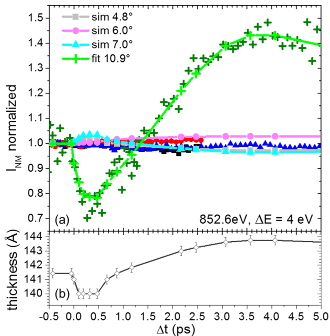
FIG. 4. (a) Comparison between measured [dark symbols taken from Fig. 2(c) for an extended time delay] and simulated (light symbols and connecting lines) temporal evolution of the nonmagnetic reflectivity ( I_{NM} ) for an incidence angle of \theta = 4.8^\circ (black), \theta = 6.0^\circ (red), \theta = 7.0^\circ (blue), and \theta = 10.9^\circ (green). As discussed in detail in the text, all four simulations are realized with the same model, which assumes the temporal evolution of the Ni film thickness shown in panel (b).
