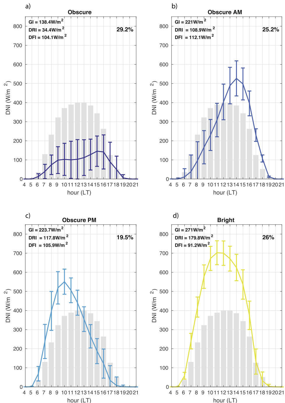
Figure 1. The four main types of diurnal cycles of the DNI. (a) Obscure, (b) obscure in the morning ('Obscure AM'), (c) obscure in the afternoon ('Obscure PM'), and (d) bright days. Coloured curves give the mean value (average over days and pixels), error bars the 0.5 std (with N = 1837\ 830/1422\ 368/1895\ 203/2128\ 900 respectively), and grey bars the overall average (all days and pixels available). In bold, the frequency of occurrence (in %) of each type over the study period (2005–2013) and the mean daily values of global (GI), direct (DRI) and diffuse (DFI) irradiances.
