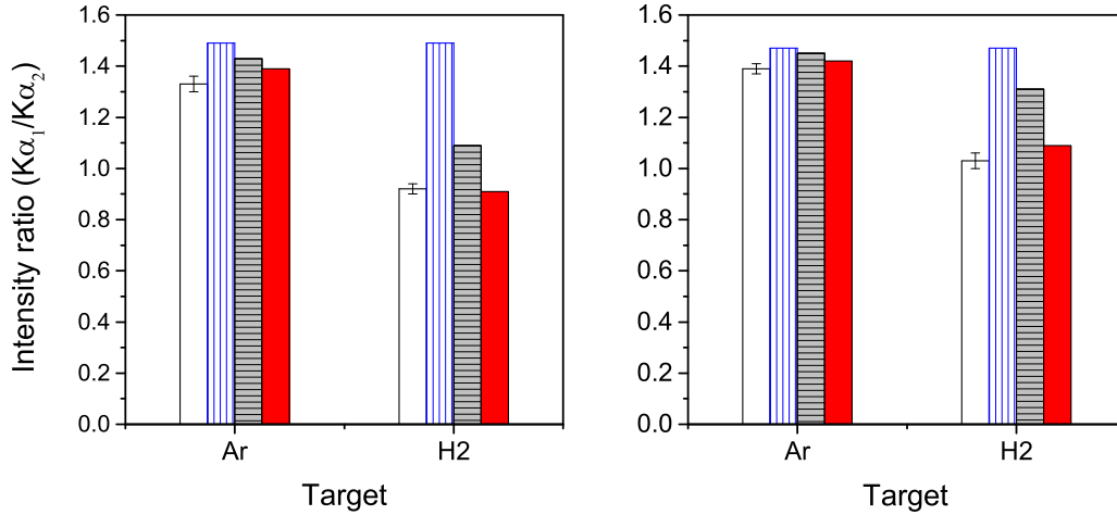
FIG. 4. Experimental results (white columns) in comparison with theoretical predictions for K\alpha_1/K\alpha_2 ratios ( A_0 ) for the K-shell excitation of U^{90+} in collisions with Ar and H_2 targets at 218 (left) and 300 MeV/ u (right). Blue columns with vertical stripes show PIE results. Solid red columns depict combined (PIE+EIE) calculations. In addition, the combined calculations without inclusion of the GBI are presented by gray columns with horizontal stripes.
