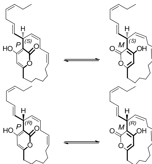
Figure 6. Structure of neurymenolide A configurations ( P, S ), ( M, S ), ( M, R ) and ( P, R ).
