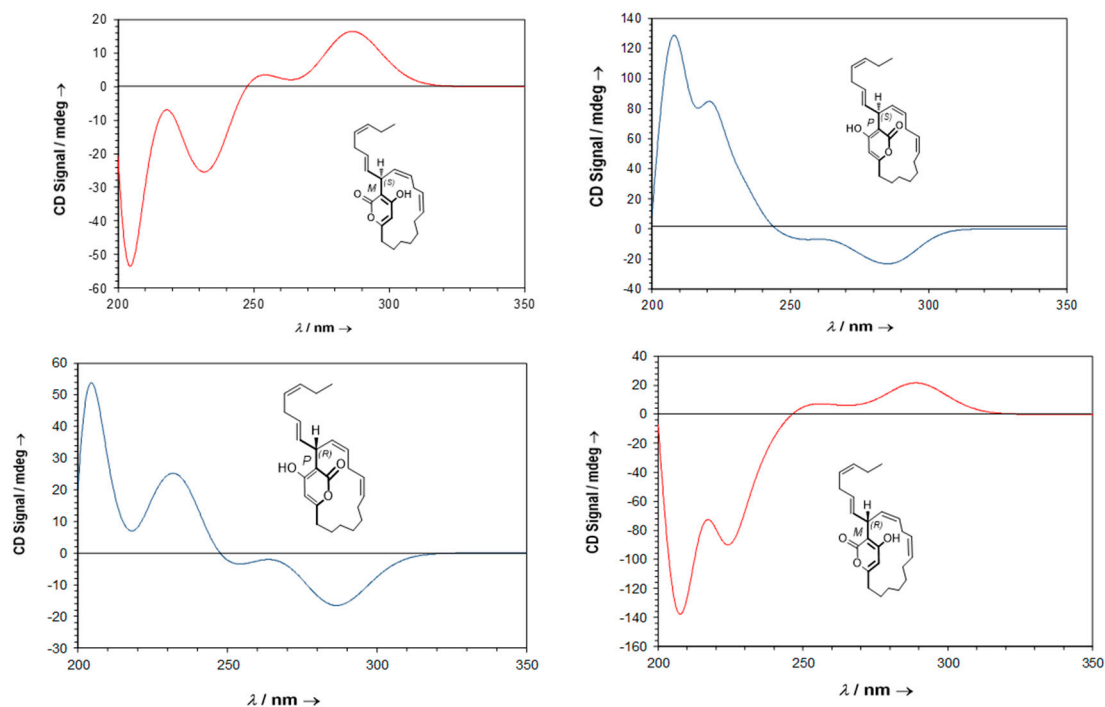
Figure 9. Theoretical ECD spectra of nearymenolide A of ( P , S ), ( M , S ), ( M , R ) and ( P , R ) configurations.
