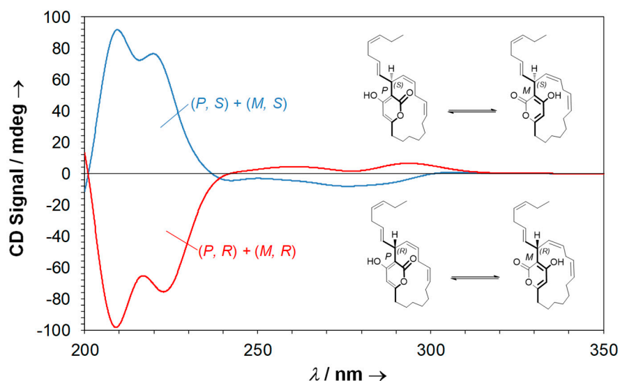
Figure 10. Theoretical ECD spectra of both possible equimolar mixtures of nearymenolide A.
