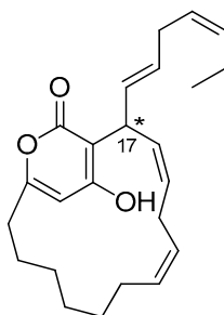
Figure 5. Structure of neurymenolide A.
