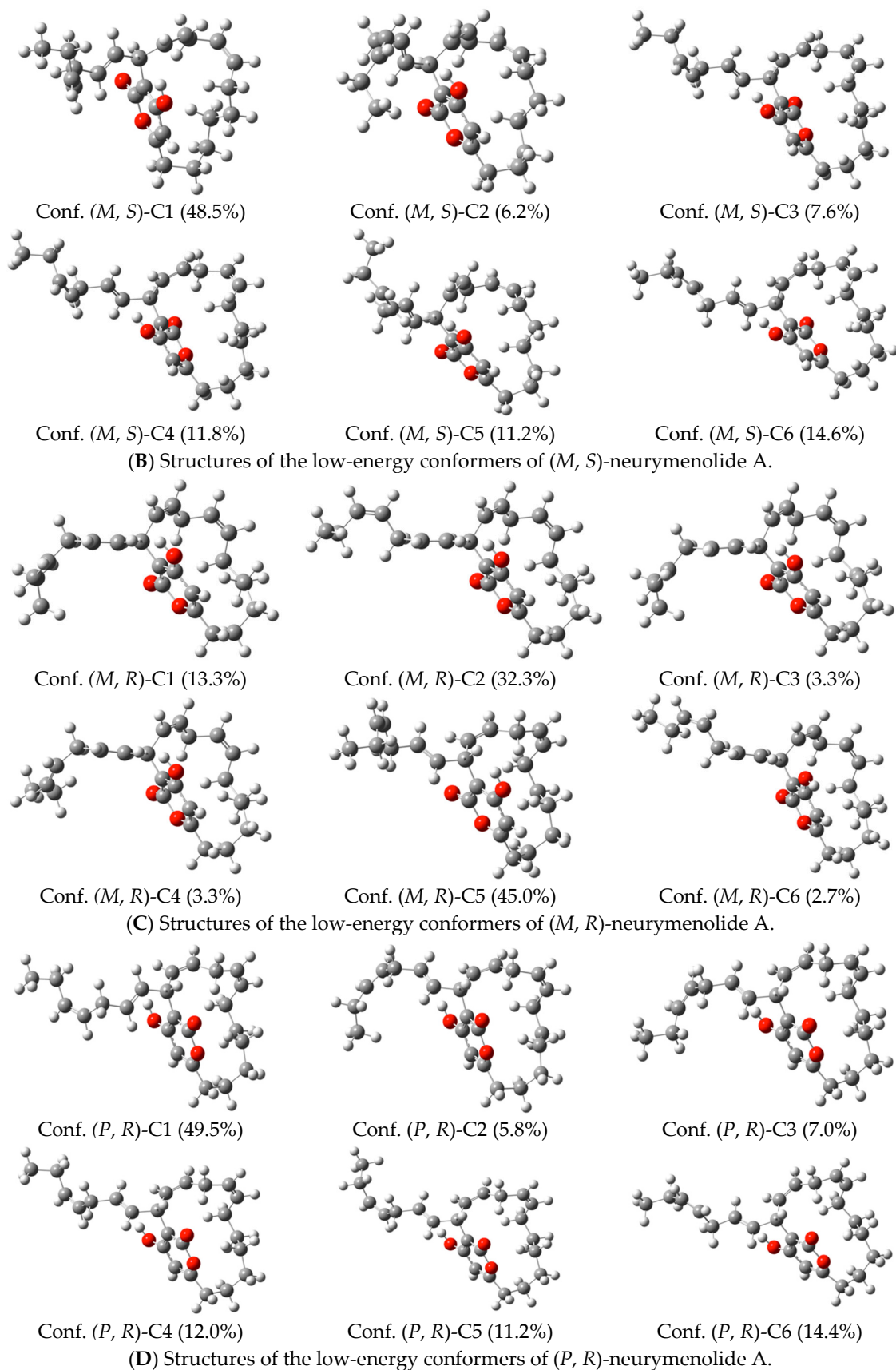
Figure 8. Structures and Boltzmann populations of the low-energy B3LYP/6-31+G(d,p) conformers (A–D) (P, S), (M, S), (M, R), and (P, R) configurations of neurymenolide A in CH 3 OH (298 K and 1 atm).
