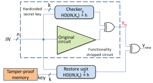
Fig. 2. SFL architecture.
