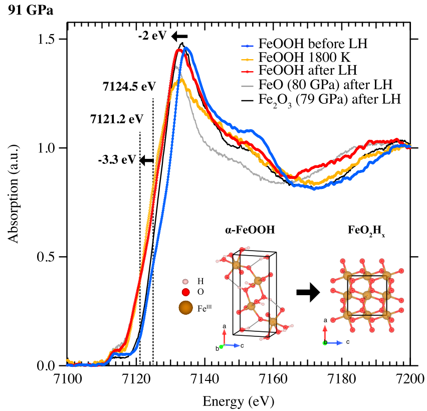
Figure 3. Normalized Fe-K edge XANES spectra collected at ~90 GPa before, during, and after laser heating (LH) of FeOOH loaded into KCl. For comparison, spectra collected in FeO and Fe 2 O 3 at similar pressure after laser heating are also represented. A shift of −3.3 eV of the Fe K-edge is observed as \alpha -FeOOH transformed into FeO 2 H x . Hydrogen atoms are not represented in the crystal structure of the FeO 2 H x .
