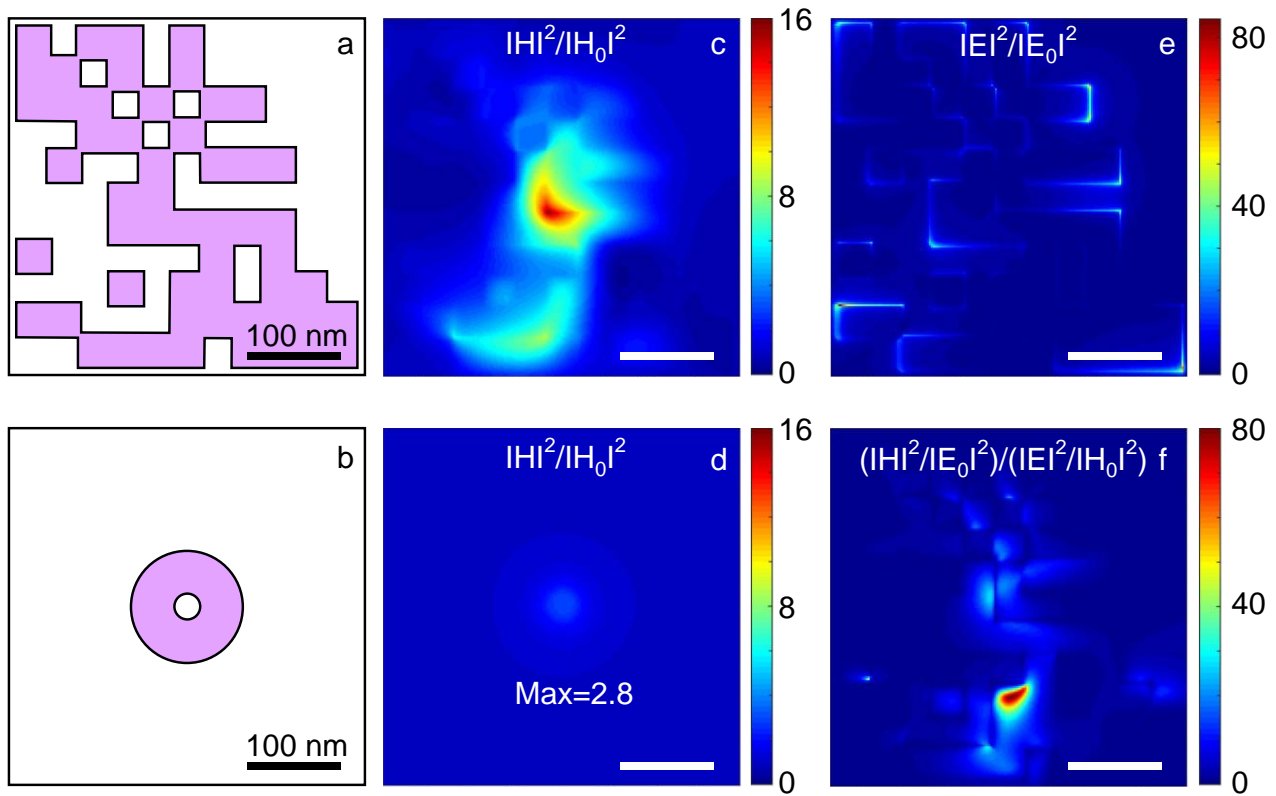
Figure 3. Optimized structure and comparison with a hollow silicon nanodisk. a) Optimized structure obtained after 248 generations and c) distribution of the magnetic intensity enhancement a) 2nm above the top plane of the antenna in z. b) Schematic of a silicon hollow nanodisk, currently considered as the best dielectric nanoantenna allowing an accessible magnetic hot spot and d) corresponding magnetic intensity increase produced by b), 2nm above the antenna in z as well, and with a maximum of 2.8. e) Electric field intensity enhancement distribution in the same plane as c. f) Magnetic over electric intensity enhancements in the same plane as c and e.
