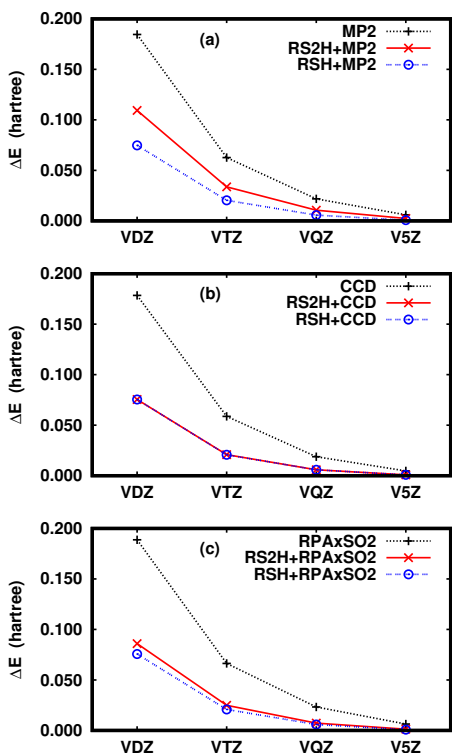
FIG. 2: Convergence of the total energy with respect to the size of basis set for the Ne atom, as measured by the basis error with respect to the V6Z basis set, \Delta E = E_{VXZ} - E_{V6Z} , where VXZ stands for cc-pVXZ with X = 2 (D), 3 (T), 4 (Q), 5, calculated with (a) MP2, RS2H+MP2 ( \mu = 0.46 , \lambda = 0.58 ), RSH+MP2 ( \mu = 0.58 ), (b) CCD, RS2H+CCD ( \mu = 0.48 , \lambda = 0.14 ), RSH+CCD ( \mu = 0.58 ), and (c) RPAxSO2, RS2H+RPAxSO2 ( \mu = 0.48 , \lambda = 0.34 ), RSH+RPAxSO2 ( \mu = 0.60 ). The parameters ( \mu, \lambda ) used are the ones optimized on the AE6+BH6 combined set.
