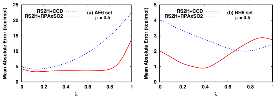
FIG. 1: MAEs for the (a) AE6 and (b) BH6 sets calculated with the RS2H+CCD and RS2H+RPAxSO2 methods as a function of \lambda for \mu = 0.5 . The basis set used is cc-pVTZ.
