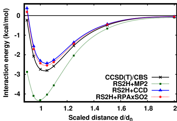
FIG. 3: Interaction energy curve of the benzene dimer in the stacked configuration calculated by RS2H+MP2 ( \mu = 0.46 , \lambda = 0.58 ), RS2H+CCD ( \mu = 0.48 , \lambda = 0.14 ), and RS2H+RPAxSO2 ( \mu = 0.48 , \lambda = 0.34 ) as a function of the scaled distance between the monomers d/d_0 where d_0 is a fixed distance. The parameters ( \mu, \lambda ) used are the ones optimized on the AE6+BH6 combined set. The counterpoise correction was applied. For RS2H+MP2, calculations were carried out using the aug-cc-pVTZ (aVTZ) basis set. For RS2H+CCD and RS2H+RPAxSO2, calculations were carried out using the aug-cc-pVDZ (aVDZ) basis set, and then the aVTZ interaction energies were estimated using E_{\text{int}}^{\text{RS2H+CCD/RPAxSO2}}(\text{aVTZ}) \approx E_{\text{int}}^{\text{RS2H+CCD/RPAxSO2}}(\text{aVDZ}) + [E_{\text{int}}^{\text{RS2H+MP2}}(\text{aVTZ}) - E_{\text{int}}^{\text{RS2H+MP2}}(\text{aVDZ})] where the RS2H+MP2 calculations are here performed with the same parameters ( \mu, \lambda ) used for the RS2H+CCD or RS2H+RPAxSO2 method. The geometries and the CCSD(T)/CBS reference interaction energies are from the S66 \times 8 data set (item number 24) of Ref. 63.
