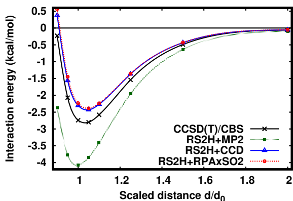
FIG. 2: Interaction energy curve of the benzene dimer in the stacked configuration calculated by RS2H+MP2, RS2H+CCD, and RS2H+RPAxSO2 as a function of the scaled distance between the monomers d/d_0 where d_0 is a fixed distance. The calculations were carried out using the aug-cc-pVDZ basis set with the counterpoise correction and using the parameters (\mu, \lambda) optimized on the AE6+BH6 combined set. The geometries and the CCSD(T)/CBS reference interaction energies are from the S66 \times 8 data set (item number 24) of Ref. 63.
