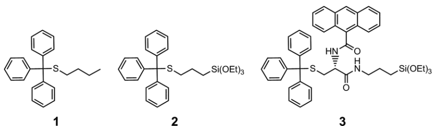
Figure 1. Molecular structures synthesized from an alkyl- S -trityl moiety (see compound 1 ), in combination with a triethoxysilane group (see compound 2 ), and belonging to a cysteine functionalized with an anthracene (see compound 3 ).
