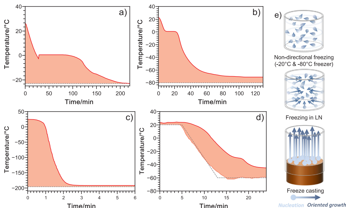
Fig. 1. Temperature profiles during freezing of 40\text{ g}\cdot\text{L}^{-1} pectin solutions using different ice templating conditions, a) -20^{\circ}\text{C} freezer, b) -80^{\circ}\text{C} freezer, c) liquid nitrogen (LN, -196^{\circ}\text{C} ), d) freeze casting at 10^{\circ}\text{C}\cdot\text{min}^{-1} ( -60^{\circ}\text{C} ). Full red line is the temperature at the core of the sample, full pale pink line is the temperature at the interface between the copper rod and the sample (for the freeze casting setup) and dashed line represents the target temperature. d) Schematic representation of ice growth for the different freezing processes. (For interpretation of the references to colour in this figure legend, the reader is referred to the web version of this article.)
