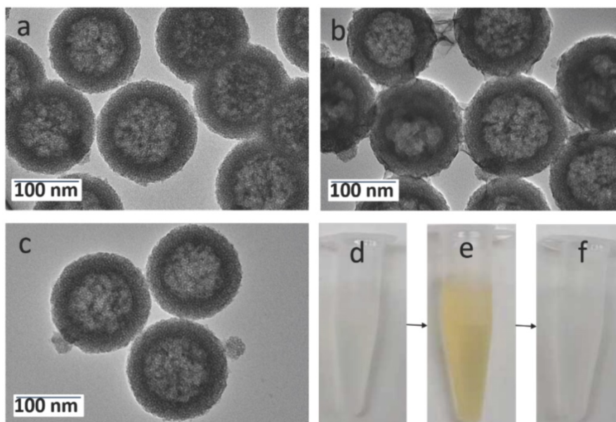
Figure 2. TEM images of (a) HMSNs, (b) HMSN@MnO 2 /apt, (c) HMSN@MnO 2 /apt after GSH treatment and the corresponding digital images from left to right (d, e, f).
