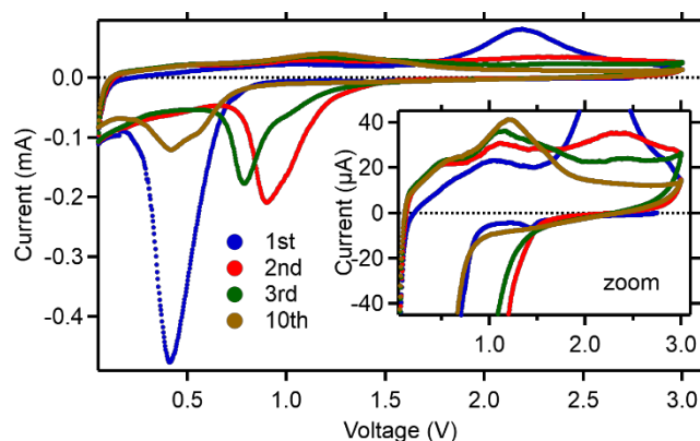
Figure 9. Cyclic voltammetry ( 0.05 - 3 V at 0.04 \text{ mV} \cdot \text{s}^{-1} ) of \text{MnF}_2 electrodes prepared using sodium alginate as binder. Formulation is \text{MnF}_2 :carbon black:Na-Alginate 8:1:1 wt. %.
