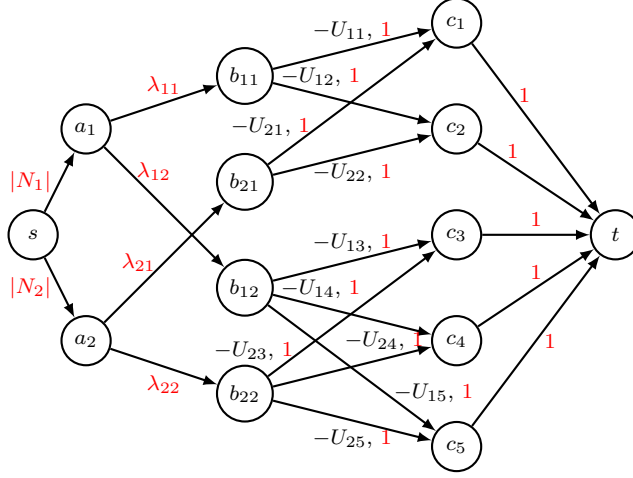
Figure 5: Network flow constructed for the proof of Theorem 4; in this case, we have 2 types and 2 blocks: M_1 = \{1, 2\} and M_2 = \{3, 4, 5\} . Arc capacities are given in red. All arcs have a cost of 0, except those between b_{pq} \in B and c_j \in C whose cost equals -U_{pj} .
