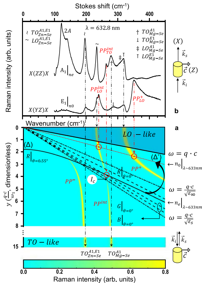
Figure 1. Near-forward-scattering Raman study of the Zn 0.74 Mg 0.26 Se VPPs. (a) The reference A 1 -like dispersion of VPPs (clear curves) including the \gamma -dependence of the Raman intensity (thickness of the curves). (b) Polarized phonon-polariton Raman spectra in the near-forward ( \theta \sim 0^\circ ) X(ZZ)X and X(YZ)X scattering geometries. In panel (a), asymptotic regimes are defined by the dispersions of light well-beneath and well-beyond the phonon resonances (dashed-dotted curves, dictated by \epsilon_\gamma and \epsilon_\infty , respectively) and by the LO's and TO's close to \Gamma and away from \Gamma , respectively. I_c refers to the photon-like extinction of the PP int mode. The dispersion within the darkened area close to \Gamma has no physical meaning. The scan lines achievable experimentally by using the effective refractive index ( n_{eff} ) in the perfect forward scattering geometry ( \theta = 0^\circ ) with the red (R, 632.8 nm), green (G, 514.5 nm) and blue (B, 488.0 nm) laser lines are indicated (dashed curves), for reference purpose. The scan line corresponding to the experimental A 1 -like X(ZZ)X Raman spectrum displayed in panel (b) is shown ( \theta = 0.55^\circ ). The curved arrow indicates an apparent upward-tilt of the corresponding scan line when shifting to the E 1 -like X(YZ)X geometry.
