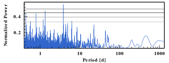
Fig. 3. Periodogram of the SOPHIE RVs for Gl 378, obtained using template-matching, and corrected for the nightly drift and the long-term variations of the zero-point. The horizontal lines indicate the 50, 10, 1, and 0.1% FAP levels (from bottom to top).
