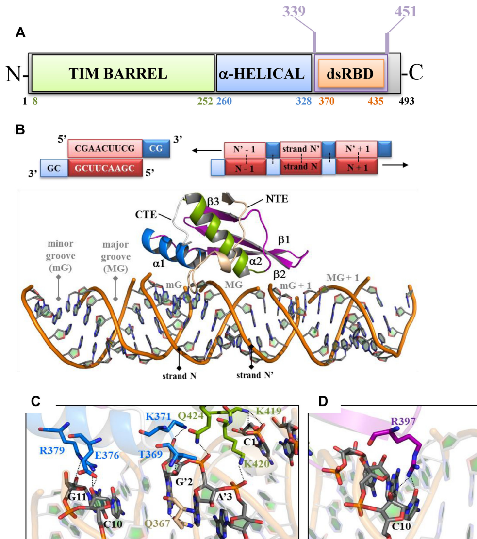
Figure 1. Mapping dsRBD residues involved in dsRNA recognition by X-ray crystallography. (A) Domain modularity of hDus2. In green is the TIM Barrel domain (TBD), which carries FMN, \alpha -helical domain (HD) is in blue and the extended dsRBD is in purple. Within the latter, there is the canonical dsRBD in orange. (B) On top is shown the RNA palindromic sequence (5'CGAACUUCGCG3') containing two overhang nucleotides used to generate a dsRNA by self-hybridization. The schematic representation of RNA palindromic sequence and two overhang nucleosides are shown as red and blue boxes, respectively. The 3'-5' RNA and its 5'-3' complementary strand are denoted as N and N' respectively. Dots show the hybridization interface between two complementary sequences while the arrows indicate the 1D direction of macromolecular self-assembly of two complementary strands into a dsRNA helix-A structure. On the bottom is shown the X-ray structure of hDus2 dsRBD in complex with dsRNA. The protein is represented in cartoons wherein helix \alpha 1, \alpha 2 and \beta sheet of dsRBD are colored in blue, green and purple, respectively. The N-terminal (NTE) and C-terminal extensions (CTE) are colored in wheat and grey, respectively. dsRNA phosphodiester backbone is represented as an orange ribbon while the ribose and nucleobases are shown as sticks (gray). (C) View on the interactions between (i) residues of helix \alpha 1 (blue sticks) and NTE (wheat sticks) and nucleoside from the minor groove (mG) and helix \alpha 2 (green sticks) with nucleoside from the major groove (MG) of the dsRNA. The nitrogen, oxygen and phosphate atoms in protein or RNA are in blue, red and orange, respectively. (D) View on the interaction involving R397 (purple sticks) in the C-terminal end of the \beta 1- \beta 2 loop and nucleosides in MG + 1.
