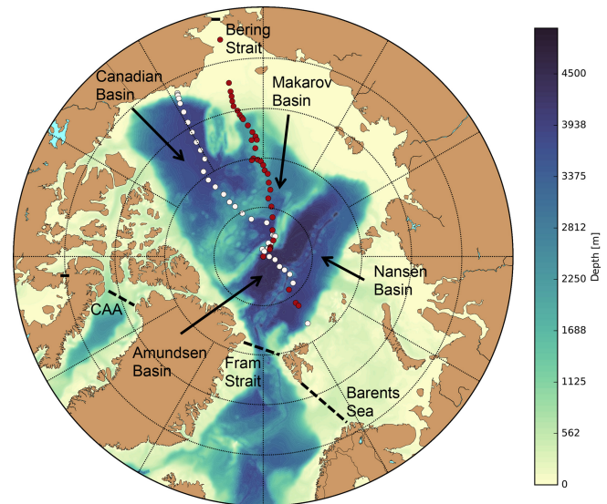
Figure 1. CFC-12 stations along the AOS94 (red) and Beringia 2005 expeditions (white). Other colors indicate the bathymetry of the Arctic Ocean, while the four dashed black lines show the boundaries of the Arctic Ocean domain used in this study.
