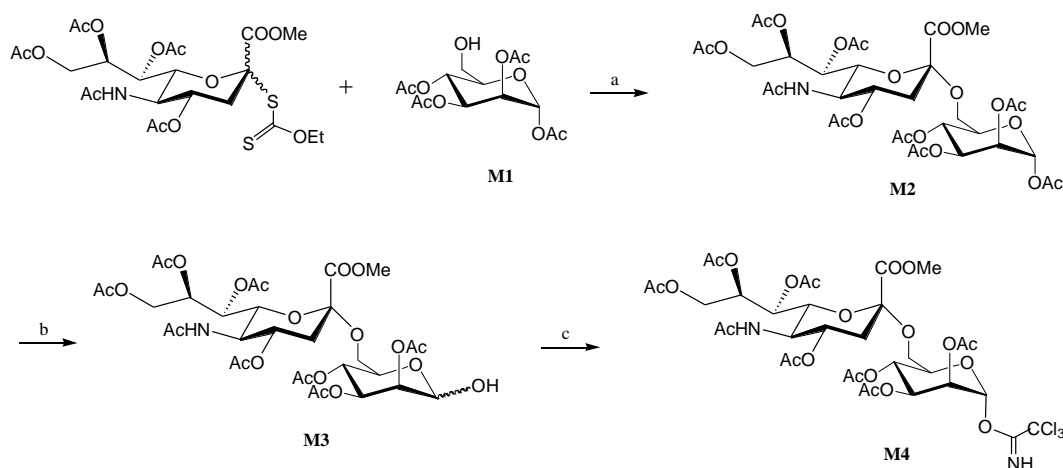
Scheme 1. Reagents and conditions: (a) \text{CH}_3\text{CN} , \text{CH}_2\text{Cl}_2 , molecular sieves, r.t., 1 h, AgOTf, DTBP, -68^\circ\text{C} , PhSCl, 3 h, 75%; (b) \text{PhCH}_2\text{NH}_2 , THF, r.t., 5 h; (c) \text{CCl}_3\text{CN} , DBU, \text{CH}_2\text{Cl}_2 , -5^\circ\text{C} , 3 h, 70% (two steps from M2).
