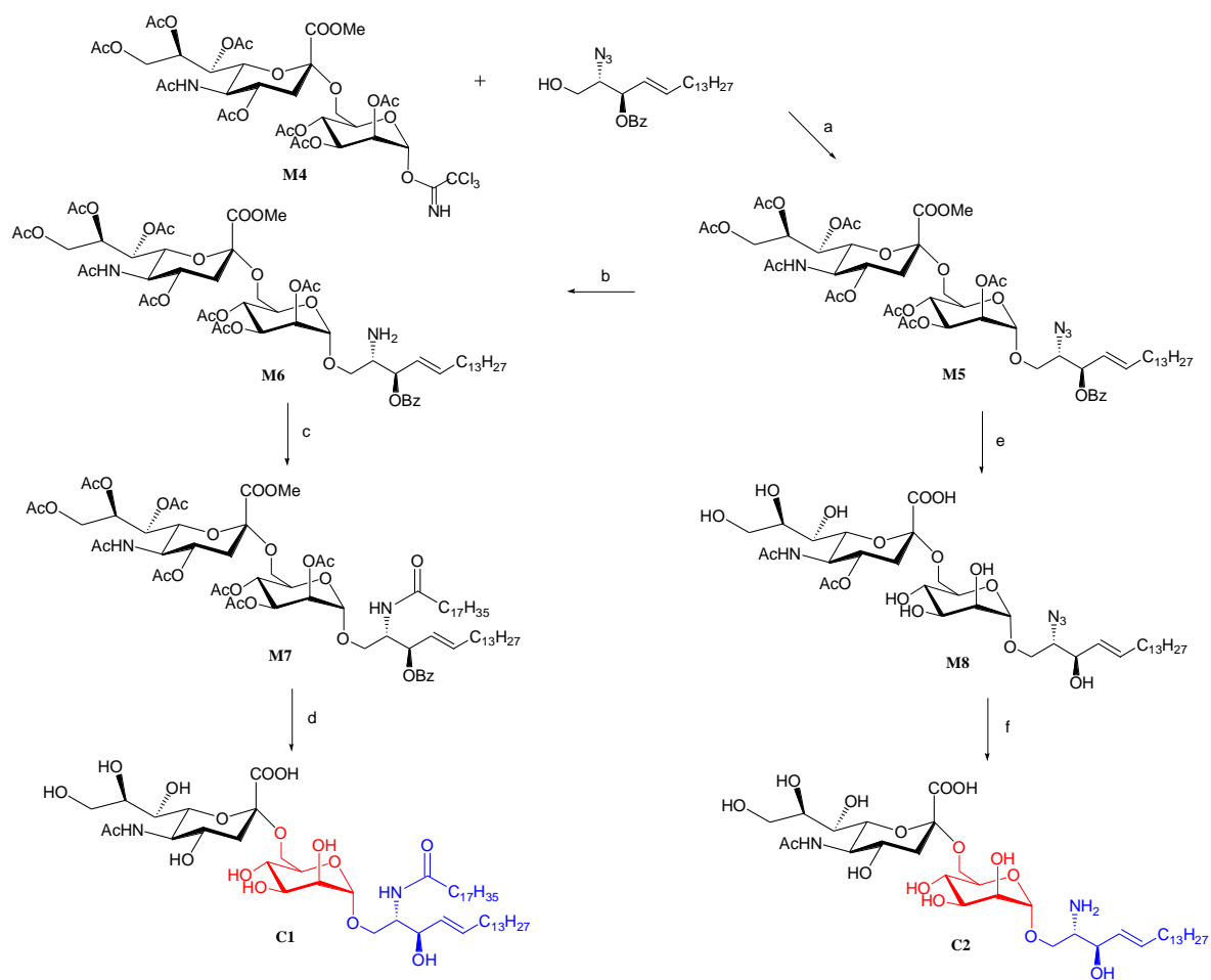
Scheme 2. Reagents and conditions: (a) \text{BF}_3\text{-Et}_2\text{O} , \text{CH}_2\text{Cl}_2 , molecular sieves, -15^\circ\text{C} , 2.5 h, 60%; (b) \text{PPh}_3 , toluene, \text{H}_2\text{O} , 50^\circ\text{C} , 12 h; (c) Stearic acid, EDC, \text{CH}_2\text{Cl}_2 , r.t., 20 h, 62% (two steps from M5); (d) \text{NaOMe} , \text{MeOH} , r.t., 14 h; \text{H}_2\text{O} , 0^\circ\text{C} , 2 h, 95%; (e) \text{NaOMe} , \text{MeOH} , r.t., 14 h; \text{H}_2\text{O} , 0^\circ\text{C} , 2 h; (f) \text{HS}(\text{CH}_2)_2\text{SH} , \text{Et}_3\text{N} , \text{MeOH} , r.t., 4 days, 80% (two steps from M5).
