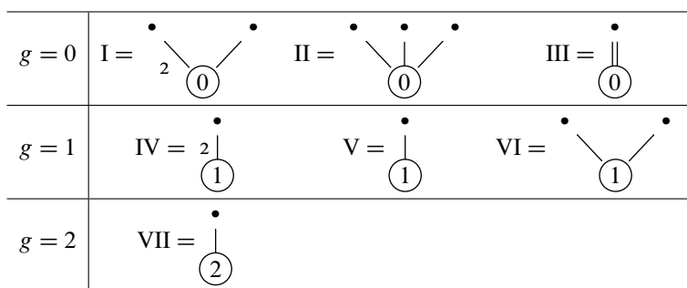
Figure 2: List of boundary terms in [\mathbb{P}\bar{A}_{g,(3)}] - (\xi + 3\psi_1)[\mathbb{P}\bar{A}_{g,(2)}]
