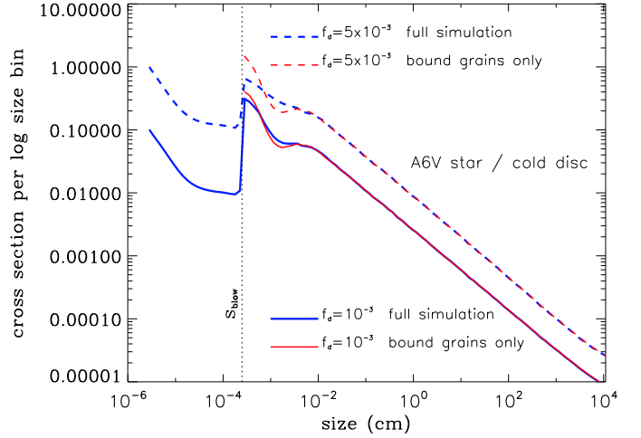
Fig. 2. Cold disc ( 50 \leq r \leq 90 au) of an A6V star: normalised disc-integrated particle size distribution at collisional steady state for a “bright” debris disc with f_d \sim 10^{-3} , and a “very bright” debris disc with f_d \sim 5 \times 10^{-3} . The red line corresponds to a simulation that only takes s \geq s_{\text{blow}} grains into account. The vertical dotted line corresponds to the blow-out size s_{\text{blow}} .
