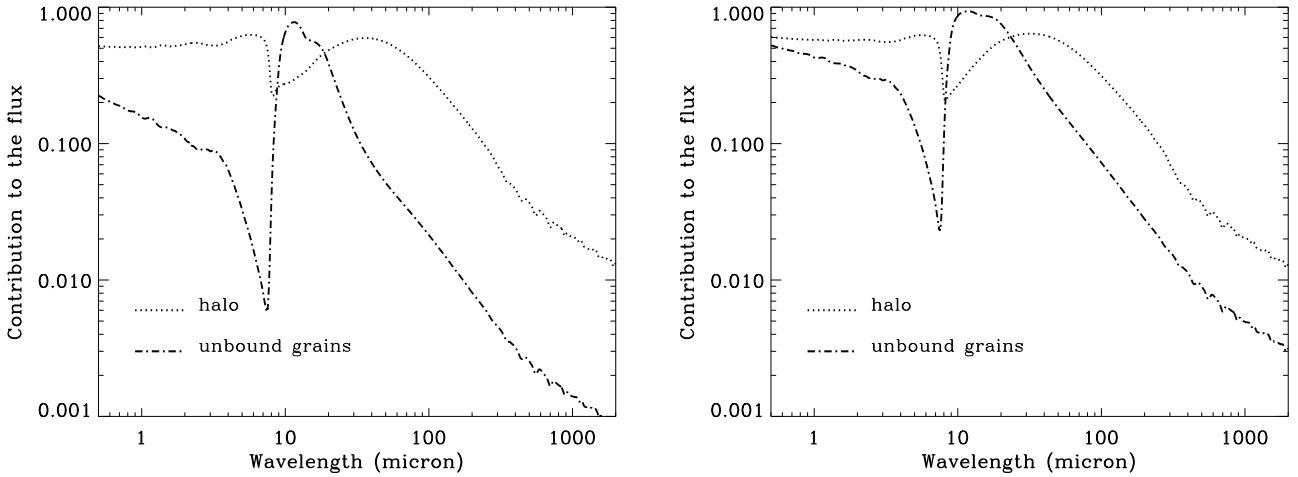
Fig. 4. Cold disk of an A6V star: fractional contribution of unbound (dash-dotted line) and halo (dotted line) grains to the SED as a function of wavelength. Left : bright debris disc with f_d \sim 10^{-3} . Right : very bright debris disc with f_d \sim 5 \times 10^{-3} .
