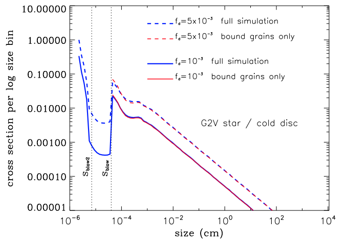
Fig. 8. Same as Fig. 2, but for a solar-type G2V star. The vertical dotted lines correspond to the two blow-out size limits s_{\text{blow}} and s_{\text{blow}2} .
