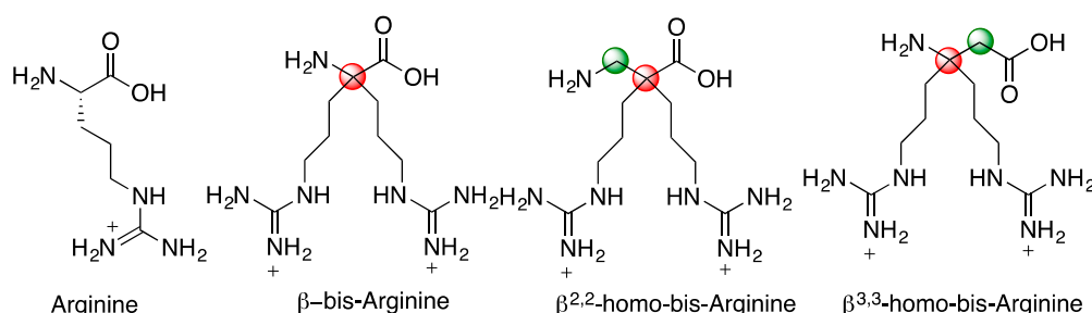
Figure 1. Bis-disubstituted-arginine analogues.
