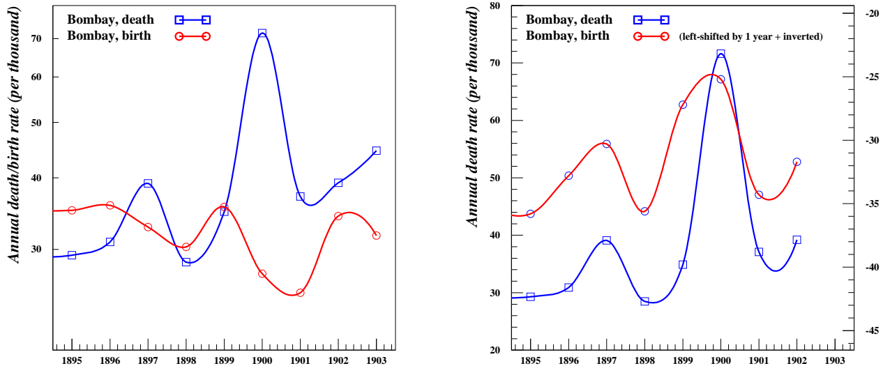
Fig. 3a,b Annual birth and death data in Bombay (1895-1903). The difference between the left- and right-hand graph is that in the later the birth series has been shifted by one year and inverted by changing its sign. There are two food crises in the time interval 1895-1903: the one of 1896–1897 which is of small magnitude and the more serious crisis of 1899-1900. The right-hand graph makes manifest that both death spikes gave rise to a birth trough in the following year. Note that in Fig.3b the y scale is linear to make the peaks more clearly visible. Source: Maharatna (1992, p.55)
