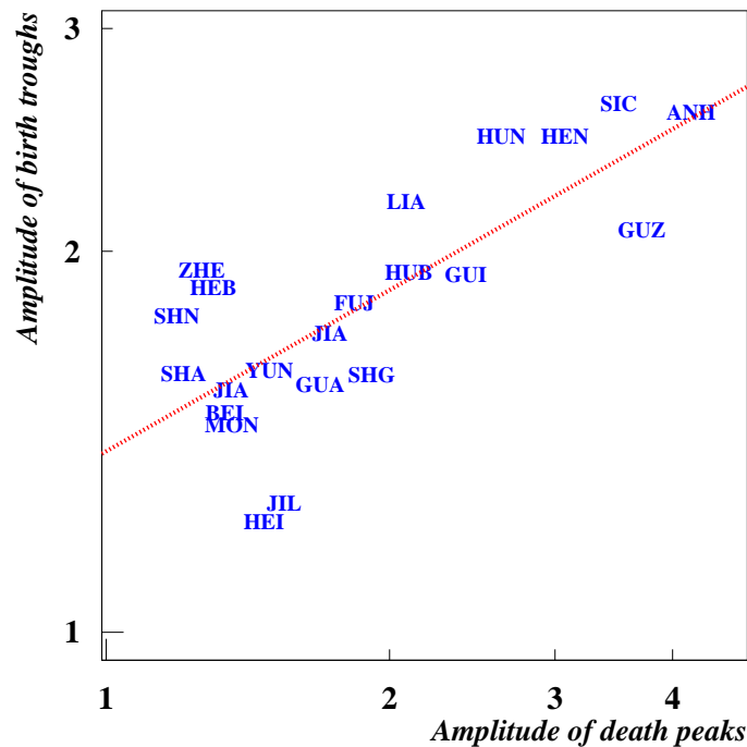
Fig. 6a China 1959-1961. Relationship between the amplitudes of death spikes and birth troughs. It is a log-log plot. The relationship between the amplitudes of the death and birth rates is as follows: A_b = CA_d^\alpha , where \alpha = 0.42 \pm 0.16 and C = 1.38 \pm 0.06 . The coefficient of linear correlation is: 0.76. The labels are the first three letters of the names of the provinces except for the following whose first three letters would have been identical: SHA=Shanxi, SHN=Shanghai, SHG=Shandong, GUA=Guangdong, GUI=Guanxi, GUZ=Guizhou. Source: Ren kou (1988)
