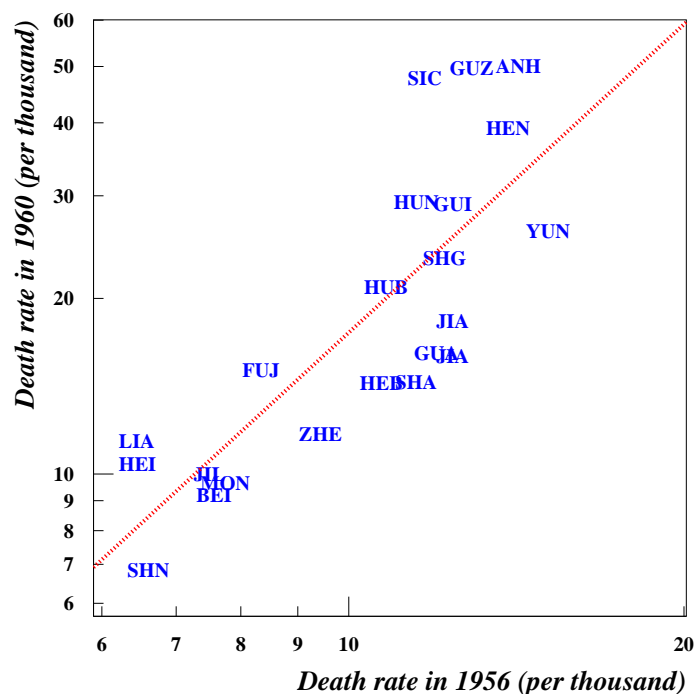
Fig. 6b Relationship between the death rates in 1956 and in 1960 (food crisis). It is a log-log plot. The coefficient of linear correlation is: 0.81. The labels are the same as in Fig.6a. Source: Ren kou (1988)
