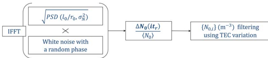
Figure 6. Spatial and temporal distribution of N_0 due to a power spectral density function.
