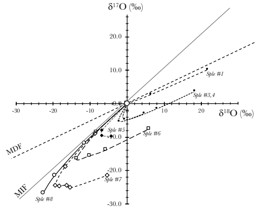
Figure 3: The isotopic compositions of O_2 are reported in the 3 isotopes diagram in \delta^{18}O units (data in Table 1). They define distillation pathways caused by the continuous removal of O_3 by its condensation at liquid nitrogen temperature on the walls of the vessel. The evolution of these pathways depends on the initial pressure of O_2 . The mass dependent ( p=0.52 ) and mass independent ( p=1 ) fractionation lines are shown for references. Note that the pathways do not define converging linear correlations.
