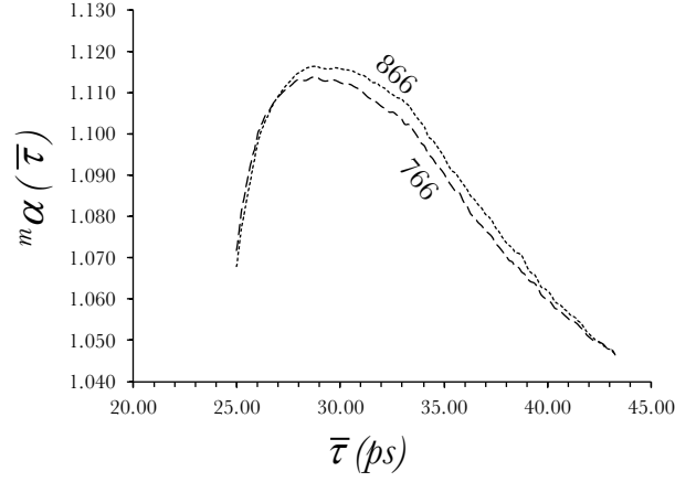
Figure 5: The mass independent isotopic fraction factors {}^m\eta(\tau) = ({}^m\text{O}/{}^{16}\text{O})_{\text{O}_3} / ({}^m\text{O}/{}^{16}\text{O})_{\text{O}_2} with m standing for mass 17 or 18 (cf. equation (17)) are reported as a function of the average lifetime \bar{\tau} of the complex \text{O}_3^* . The notations 6, 7 and 8 stand for {}^{16}\text{O} , {}^{17}\text{O} and {}^{18}\text{O} . {}^m\eta(\tau) is calculated for a scrambled mixing of the isotopomers 6-6m, 6-m-6 and m-66.
