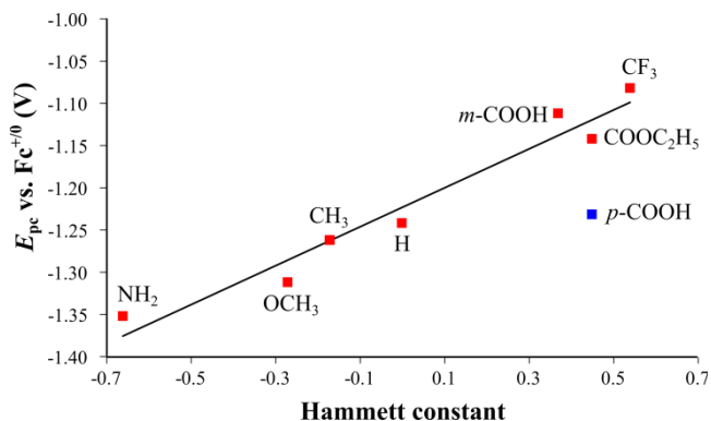
Figure 2. Trend between the electron-donating character of the bpy substituent and the first cathodic peak potential ( E_{pc} ) of complexes C1–C8 . Blue square corresponds to C6 .
