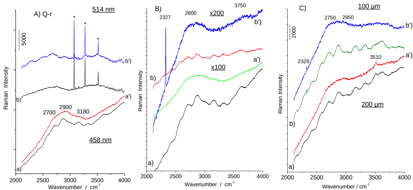
FIGURE 5 Comparison of Raman spectra recorded on the same sample with different experimental parameters: a,b: as recorded; a',b': spectra after subtraction of the waves due to the filtering. A: Spectra of Q-r obtained with green (10 mW at the sample) and blue (6 mW at the sample) lasers; B: Spectra of M-blb obtained with x200 and x100 microscope objectives; C: Spectra of T-p obtained with 100 and 200 \mu\text{m} confocal hole,
