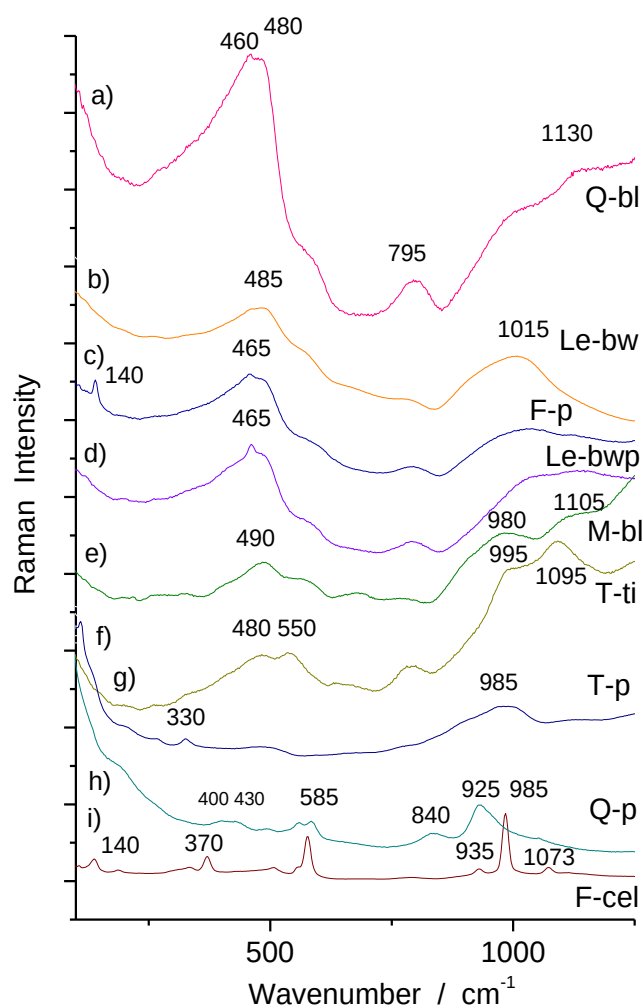
FIGURE 6 Representative Raman spectra of the different types of glazes collected from different coloured areas of the samples (x100 objective; c.h.: 200 \mu\text{m} ): a) Q-bl white, b) Lè-bw blue, c) F-p white, d) Lè-bwp white, e) M-blb blue, f) T-p yellow, g) T-ti blue, h) Q-p green, i) F-cel green (see also Table 1 for more details).
